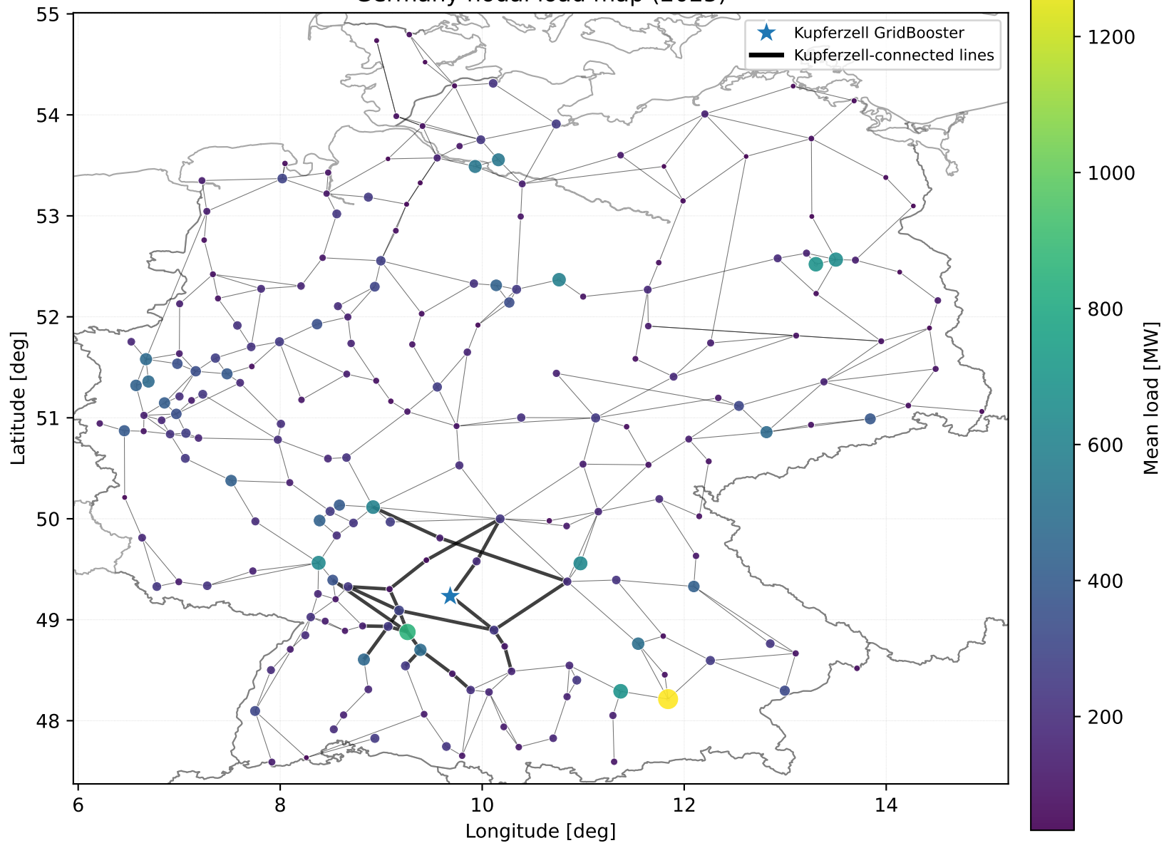
Germany nodal load map (2025)
