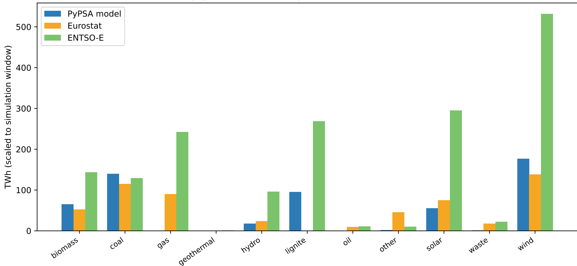
Germany generation mix — PyPSA / Eurostat / ENTSO-E (2025)
