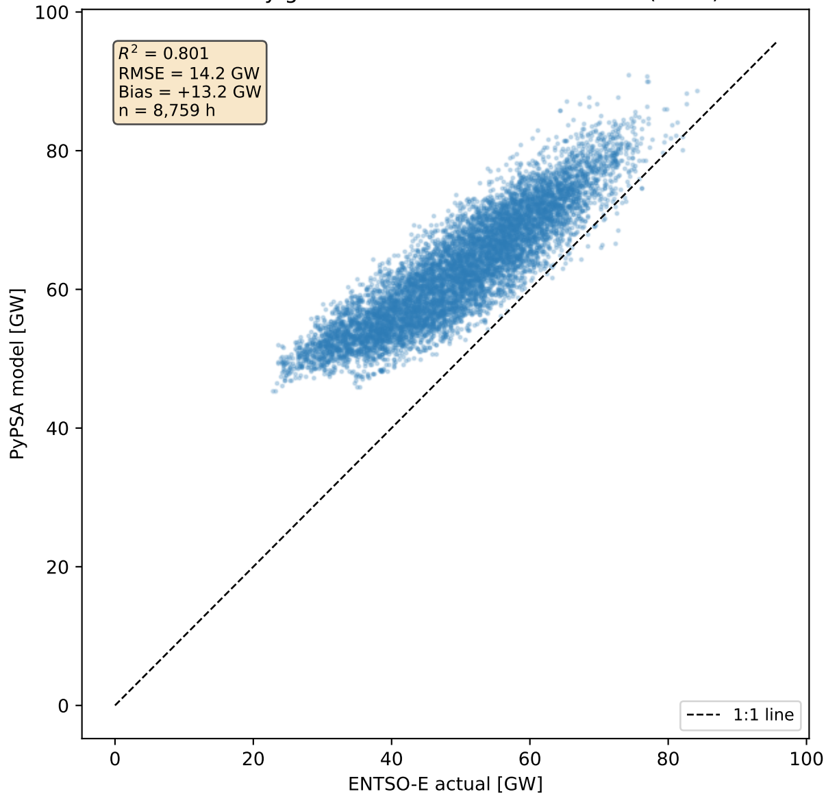
DE hourly generation — Model vs ENTSO-E (2025)
