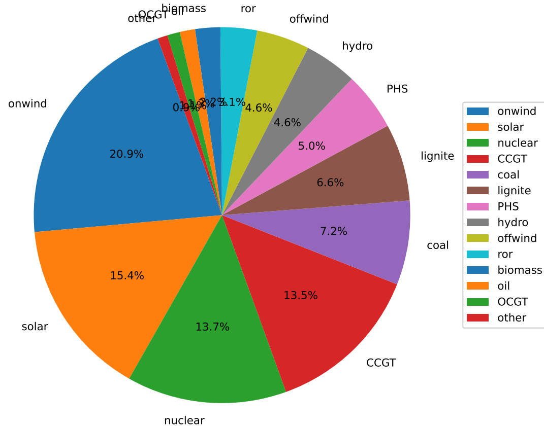
Installed capacity mix Total: 564730.74 MW
