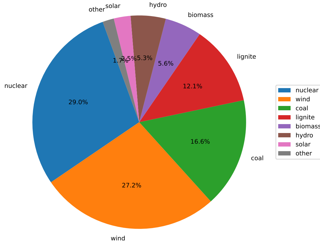
Model generation mix Total: 142.49 TWh
