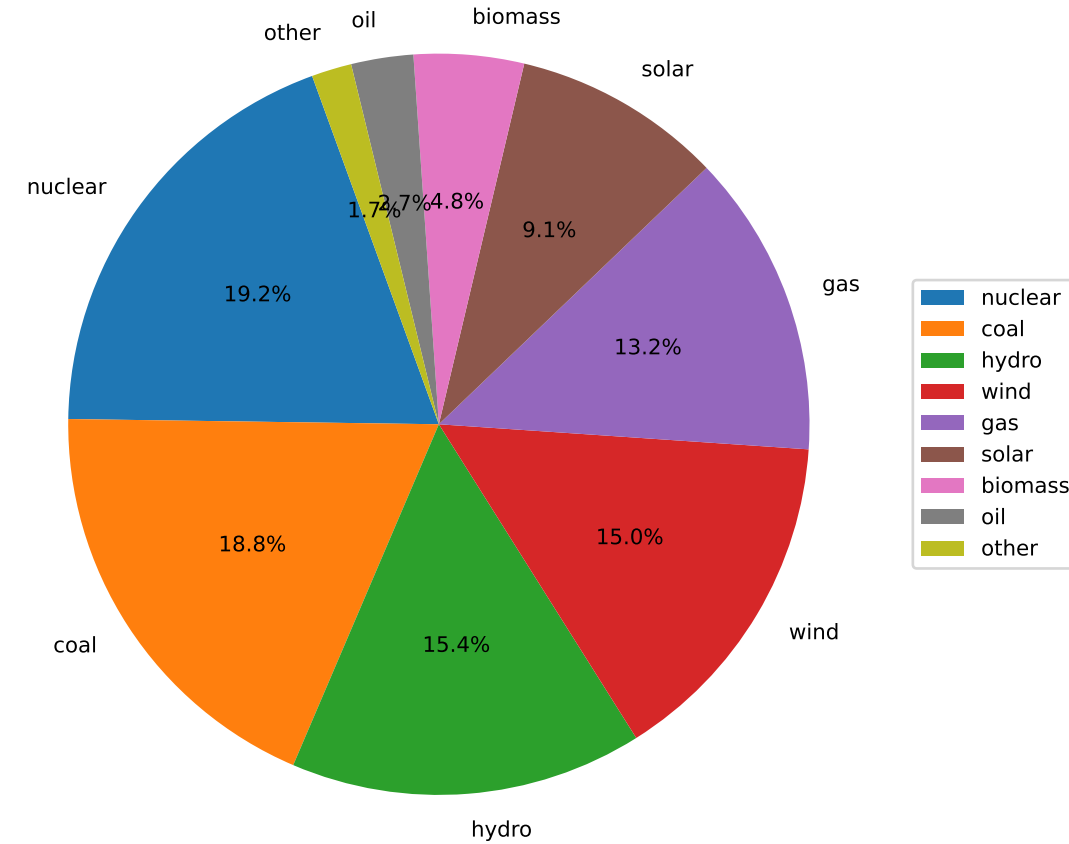
Eurostat generation mix (scaled) Total: 286.25 TWh
