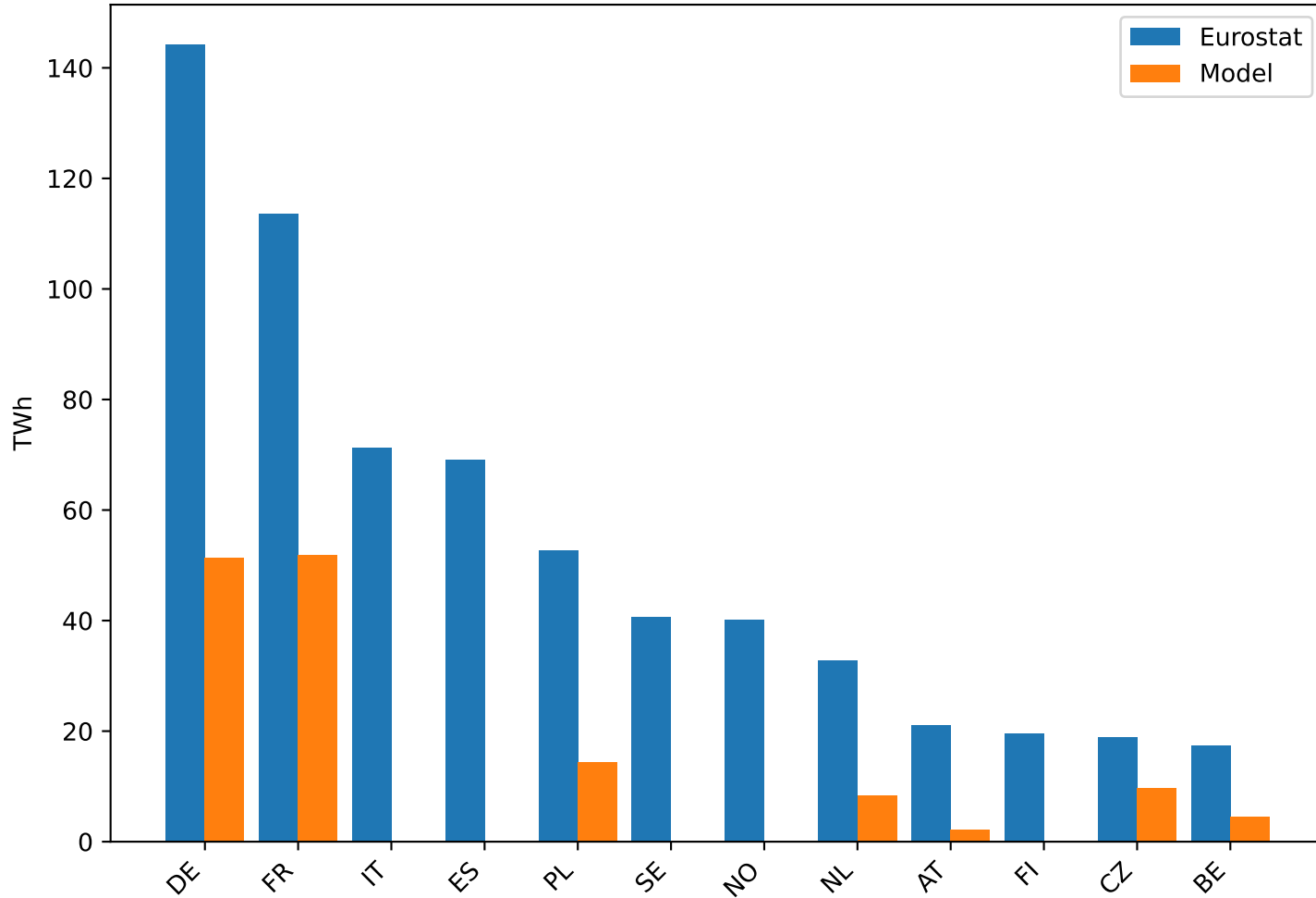
Country total generation (top by Eurostat)
