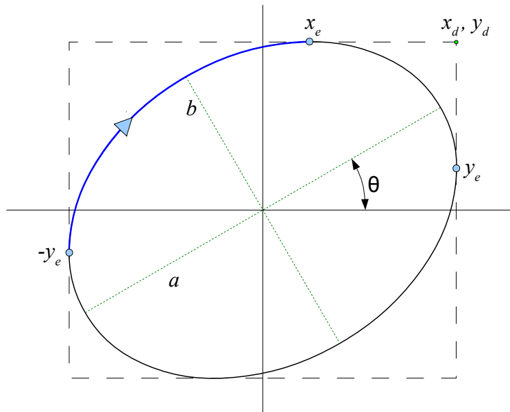
Figure 15: Rotated ellipse
