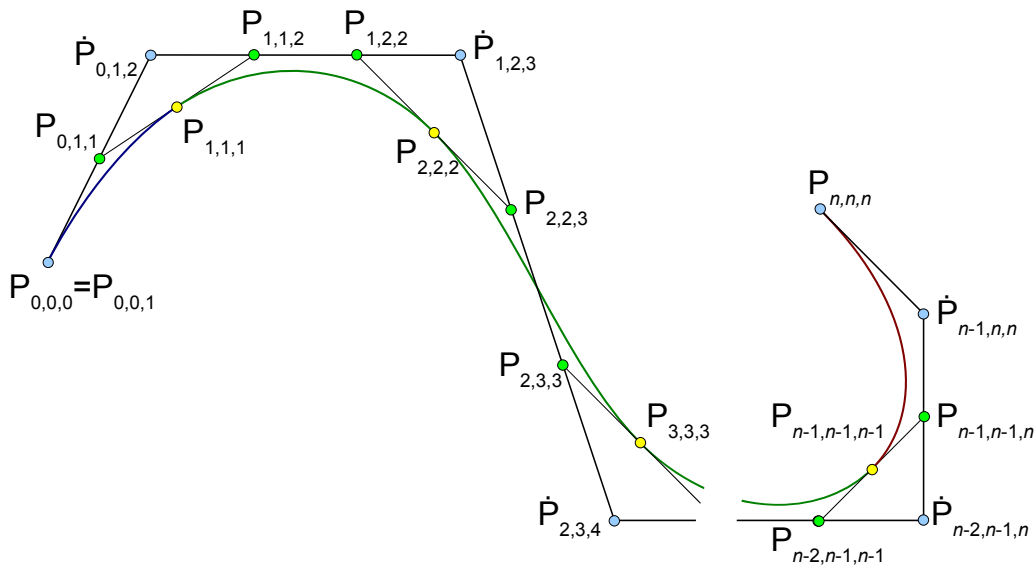
Figure 36: Cubic spline
