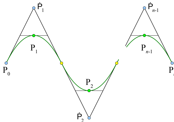
Figure 35: Quadratic spline
