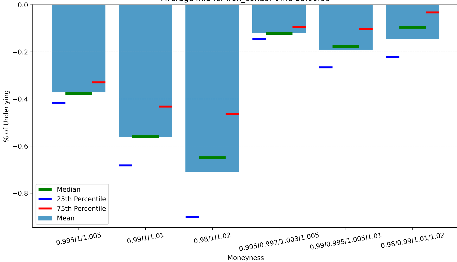
Average mid for iron_condor time 16:00:00
