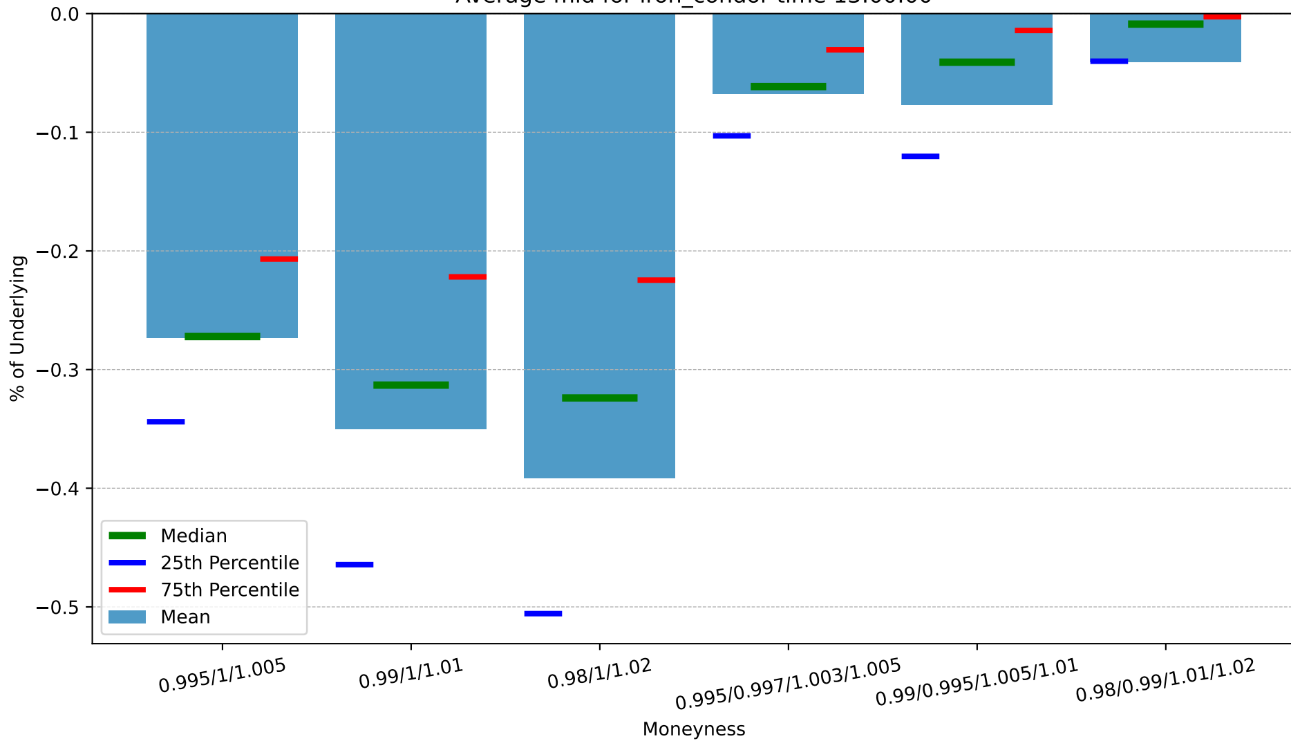
Average mid for iron_condor time 13:00:00
