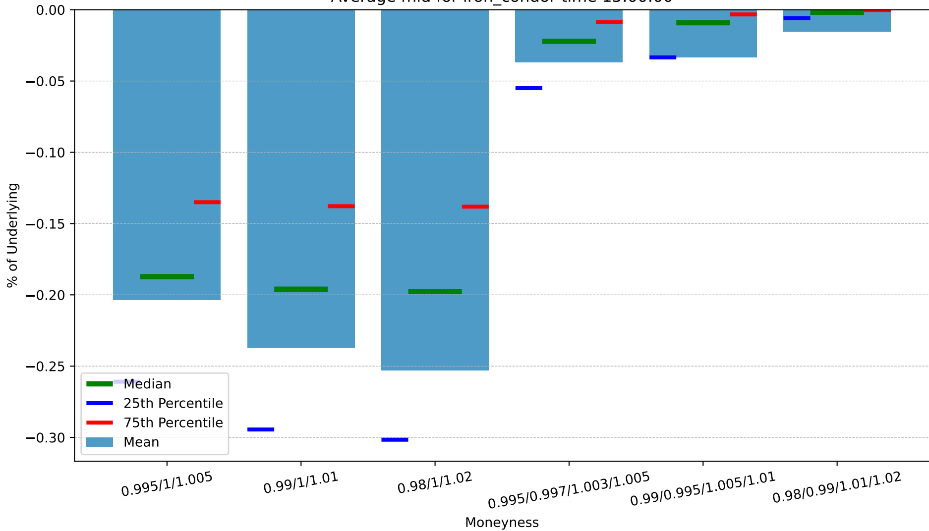
Average mid for iron_condor time 15:00:00
