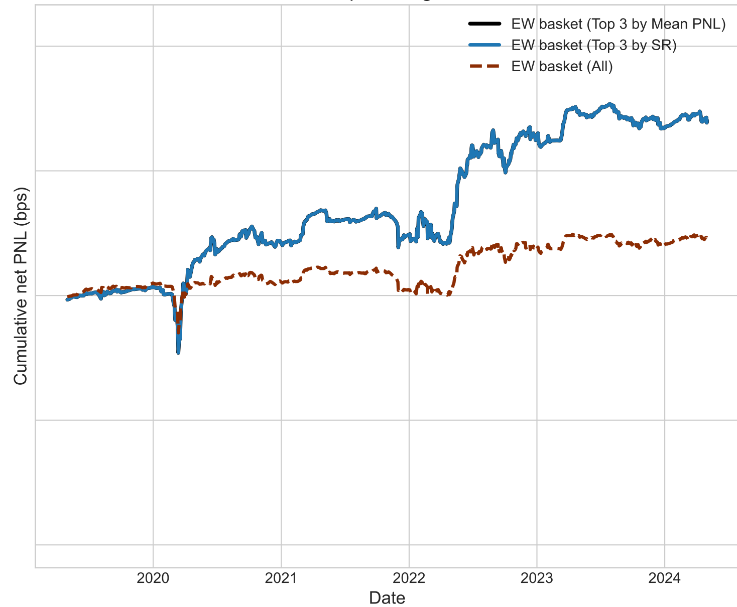
Panel B: Equal-Weight Baskets
