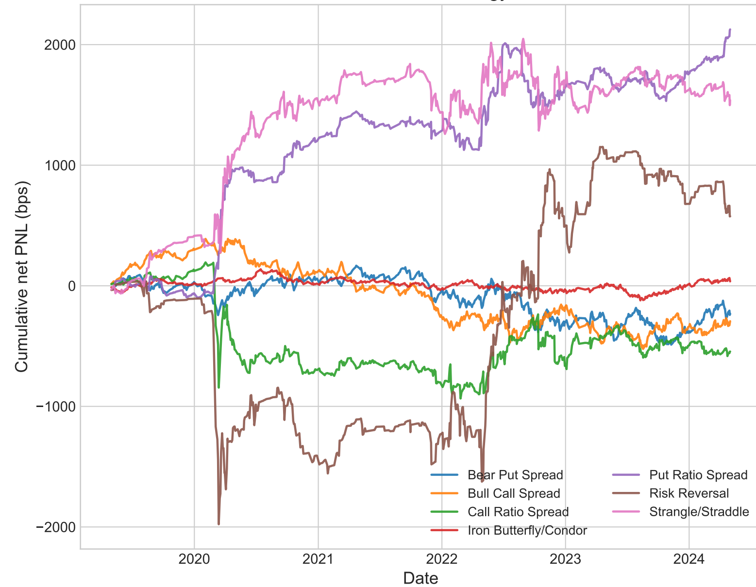
Panel A: Individual Strategy Series
