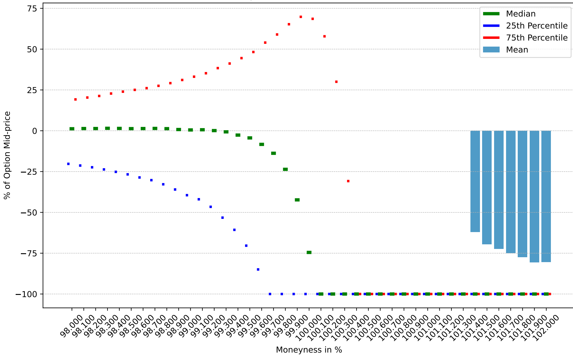
Average reth for calls time 10:00:00
