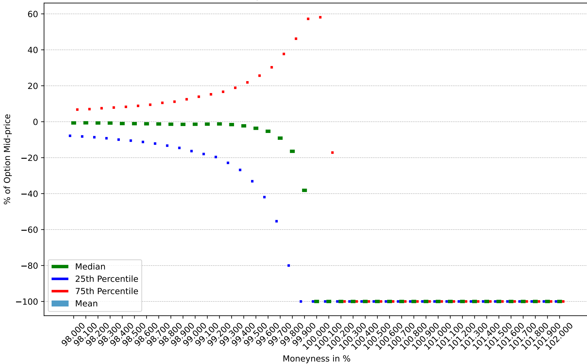
Average reth for calls time 15:00:00
