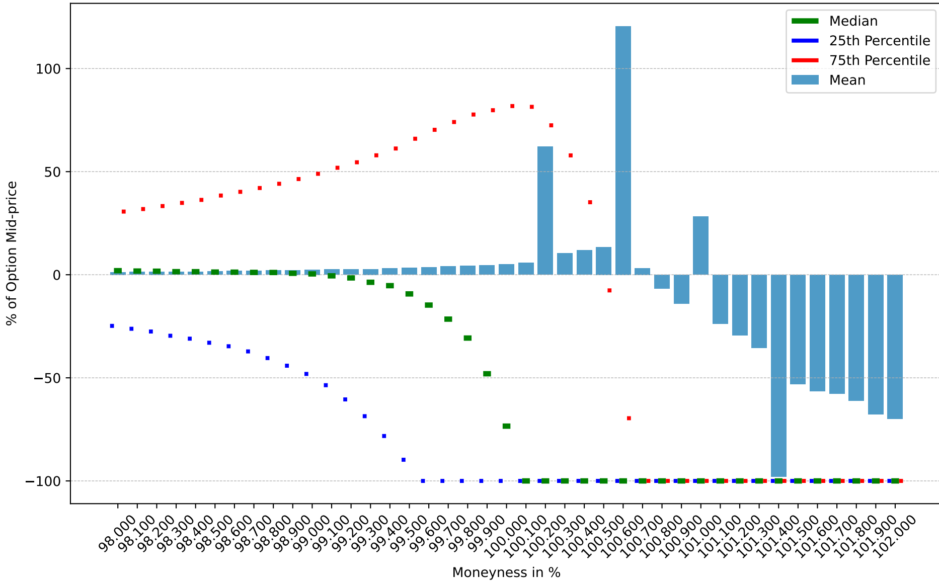
Average reth for calls time 16:00:00
