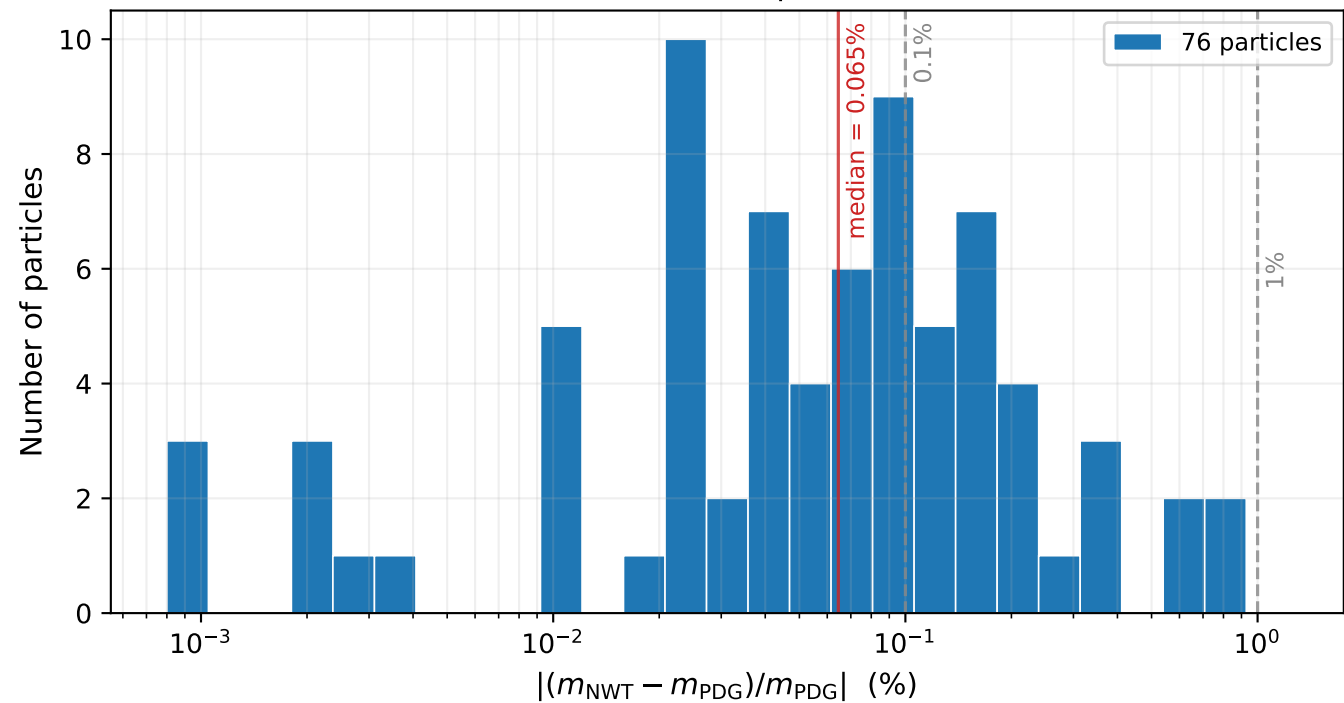
NWT residual distribution — 76 particles, median 0.065%
