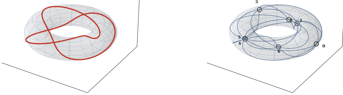
Figure 1: The two substrate objects of the gravitational program on the same Heegaard torus T^2 \subset S^3/2I . (a) The (2,3) torus knot (trefoil) is the BPS background of the matter Lagrangian introduced in Paper 16: a (p,q) winding on T^2 with mass contribution \propto p^2 + q^2 . (b) The complete graph K_7 on its Heffter triangular embedding (vertices labeled 0–6, E = 21 edges drawn as shortest-geodesic segments on the torus surface) is the Wilson-graph object of Paper 17, evaluating to the amplitude A_{K_7} = \text{bracket}(\alpha) \alpha^{21/2} . The structural identity (45), m_{\text{Pl}}^2/m_e^2 = |A_{K_7}|^{-2} , says these two objects are not two different substrate constructions but two views of one: the same toroidal background that supports the BPS trefoil also supports the K_7 graph state, and the relation between the matter-loop cutoff (a) and the IR mass hierarchy (b) is fixed by their joint embedding on T^2 .
