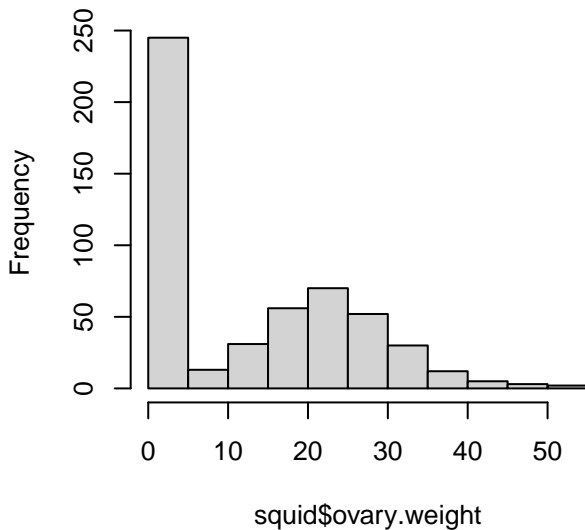
Histogram of squid$ovary.weight
