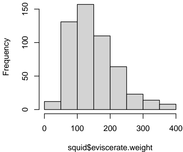
Histogram of squid$viscerate.weight
