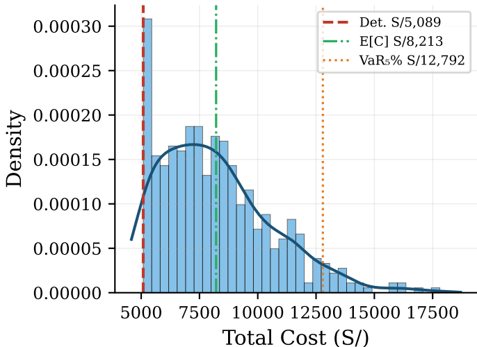
Fig. 2. Cost distribution (500 MC scenarios)
