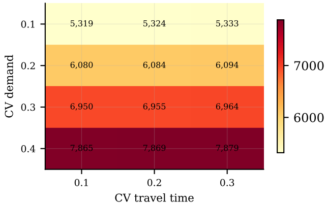
(a) E[Cost] (S/)
