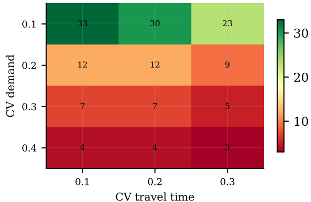
(b) Route reliability (%)
