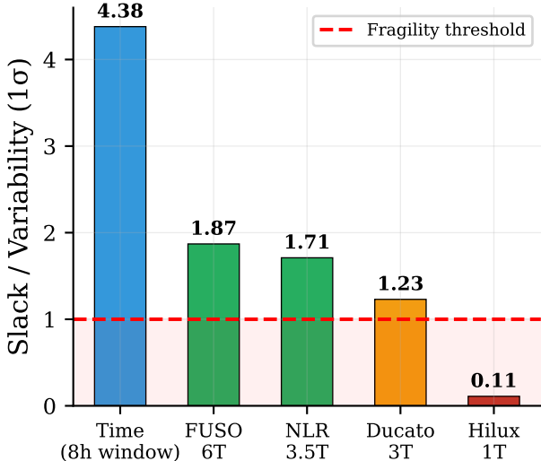
Fig. 5. Slack-to-variability ratio
