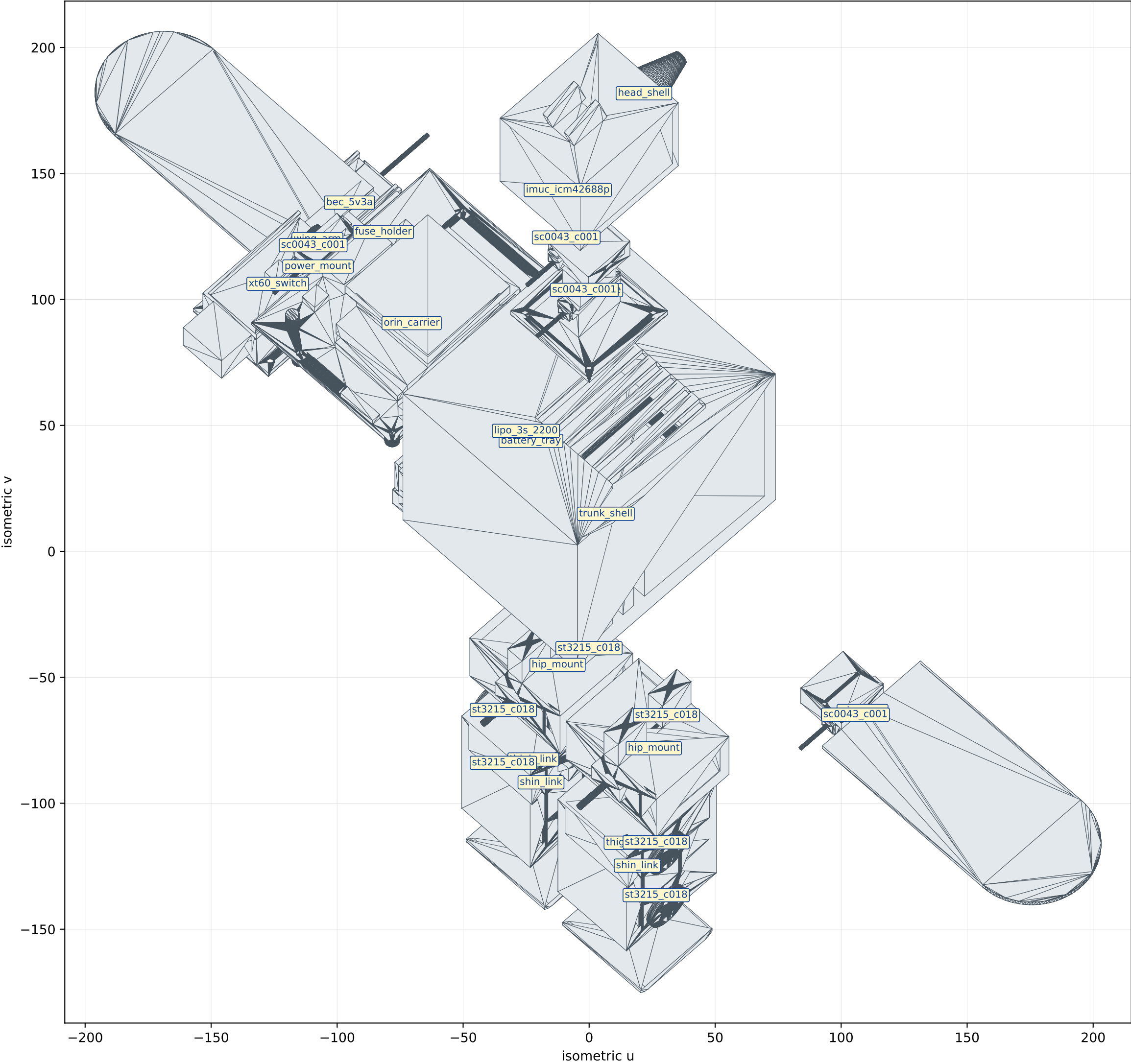
LaFengParrot — EXPLODED isometric (exploded() pose; parts separated \geq 30 mm) labels = CAD part_id (see ASSEMBLY.md 1:1 BOM map). Dimensions in mm.
