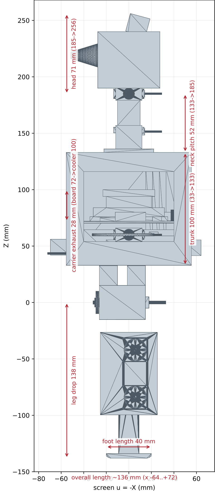
LaFengParrot - SIDE orthographic (look along +Y; -X screen-horizontal, Z up) REV-B standing zero pose, beak = screen right. Dimensions in mm.
