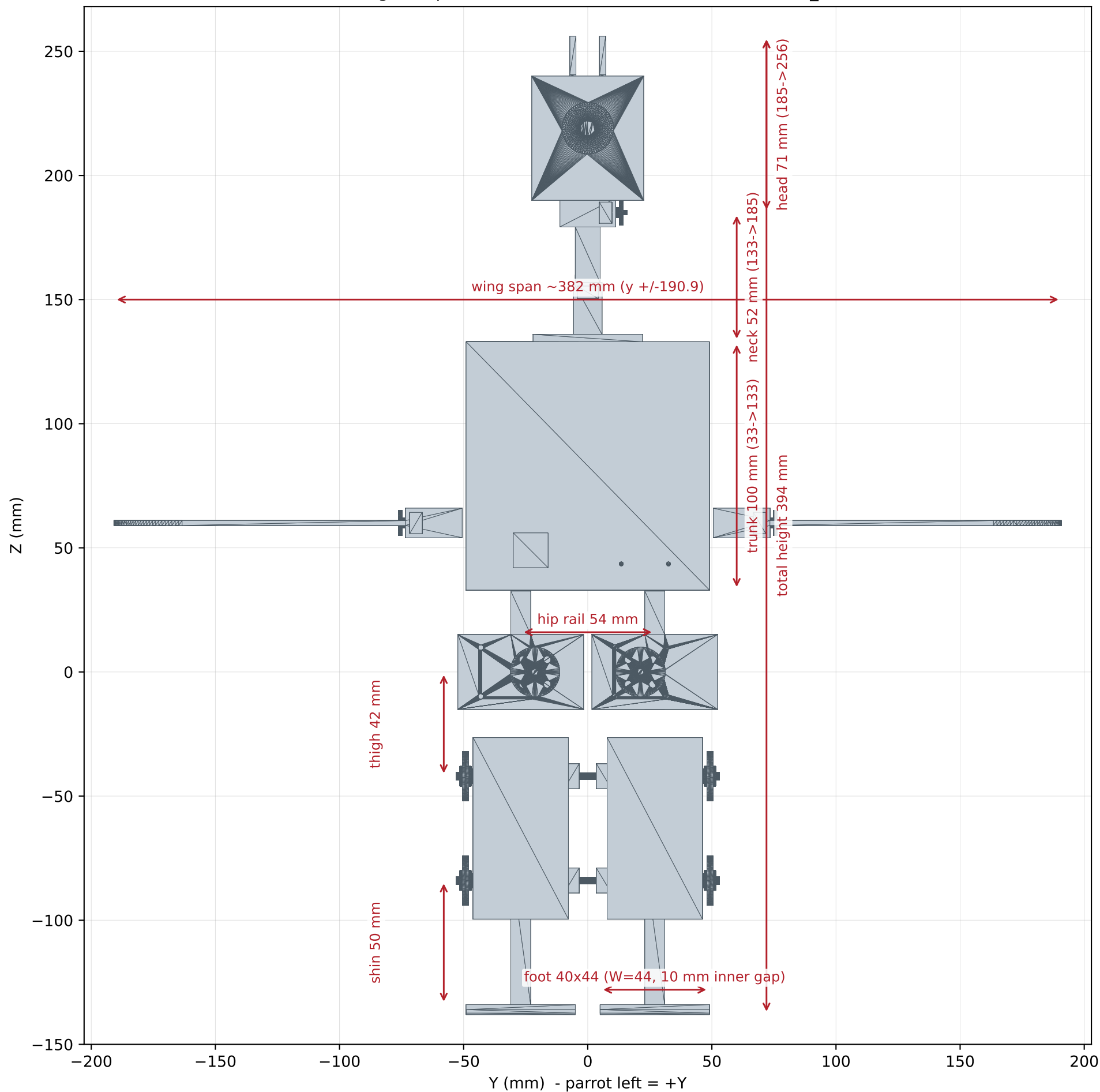
LaFengParrot - FRONT orthographic (look along +X; Y horizontal, Z up) REV-B standing zero pose, dimensions in mm. Source: ASSEMBLY_REPORT.md
