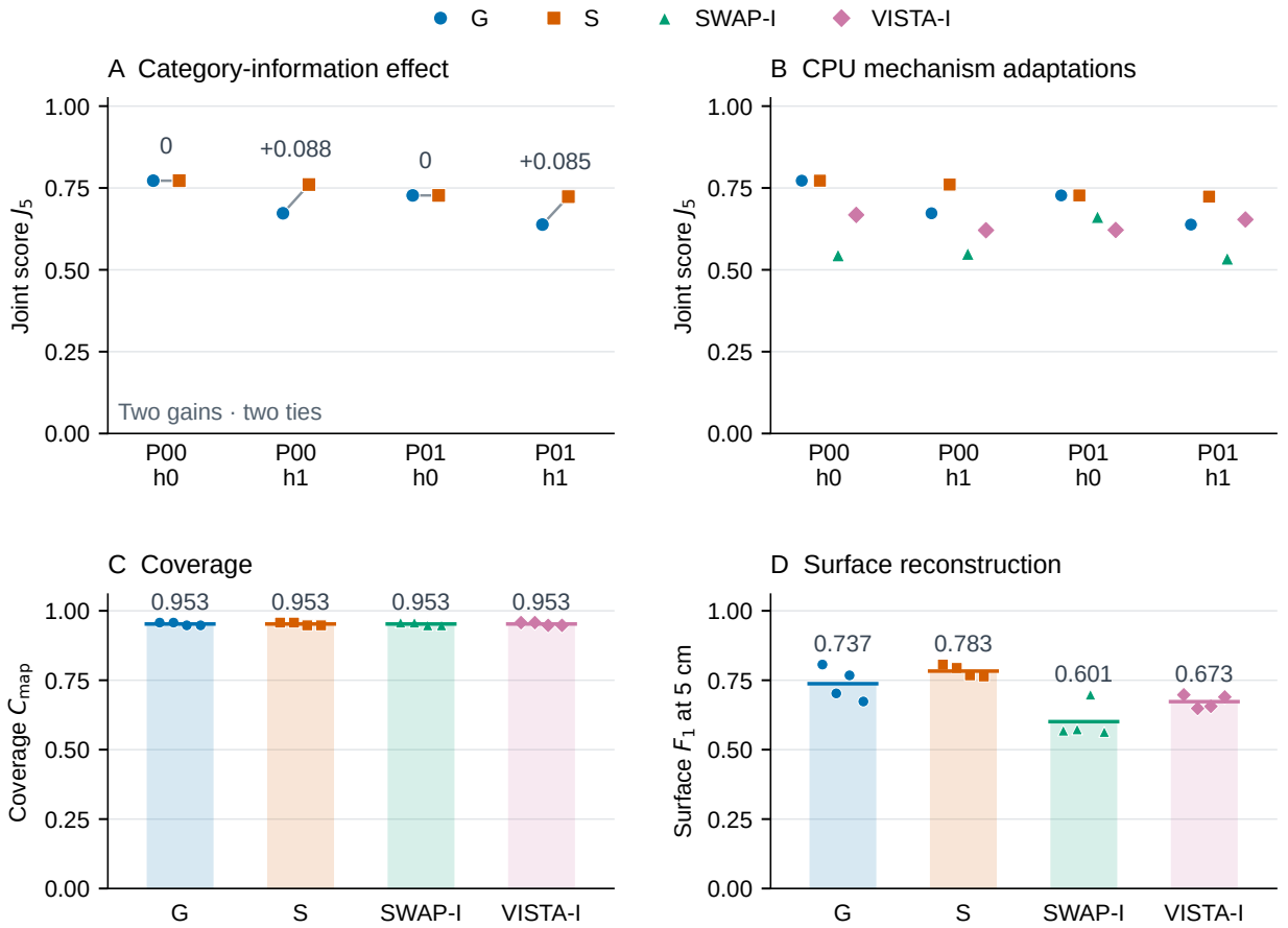
Figure 3 Complete paired outcomes, including both ties, and the coverage/F1 decomposition. Points represent conditions; horizontal caps indicate means rather than confidence intervals. G/S trajectories reused in the external-mechanism panel are not additional evidence.
