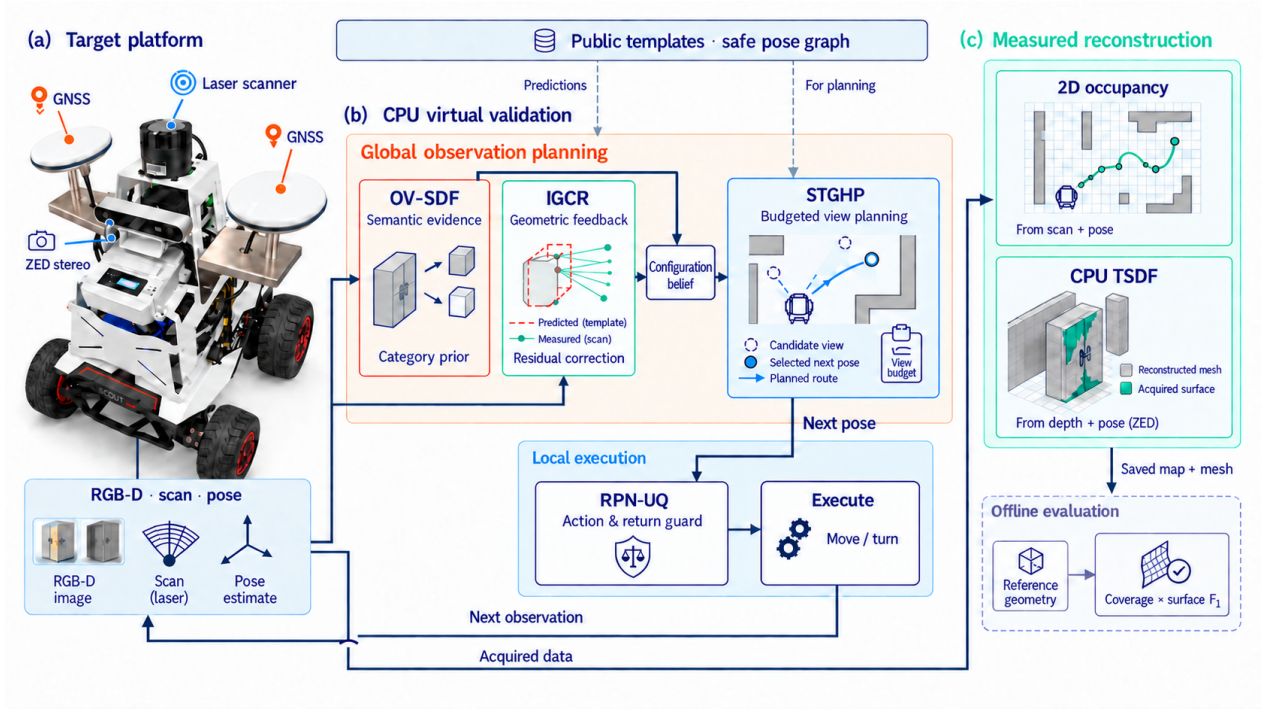
Figure 1 CPU observation and execution architecture. Category and geometric evidence update the belief used for planning; acquired depth separately enters TSDF fusion. The robot is a generative composite based on the supplied laboratory photograph, and map thumbnails are schematic. Performance results are exclusively simulated.
