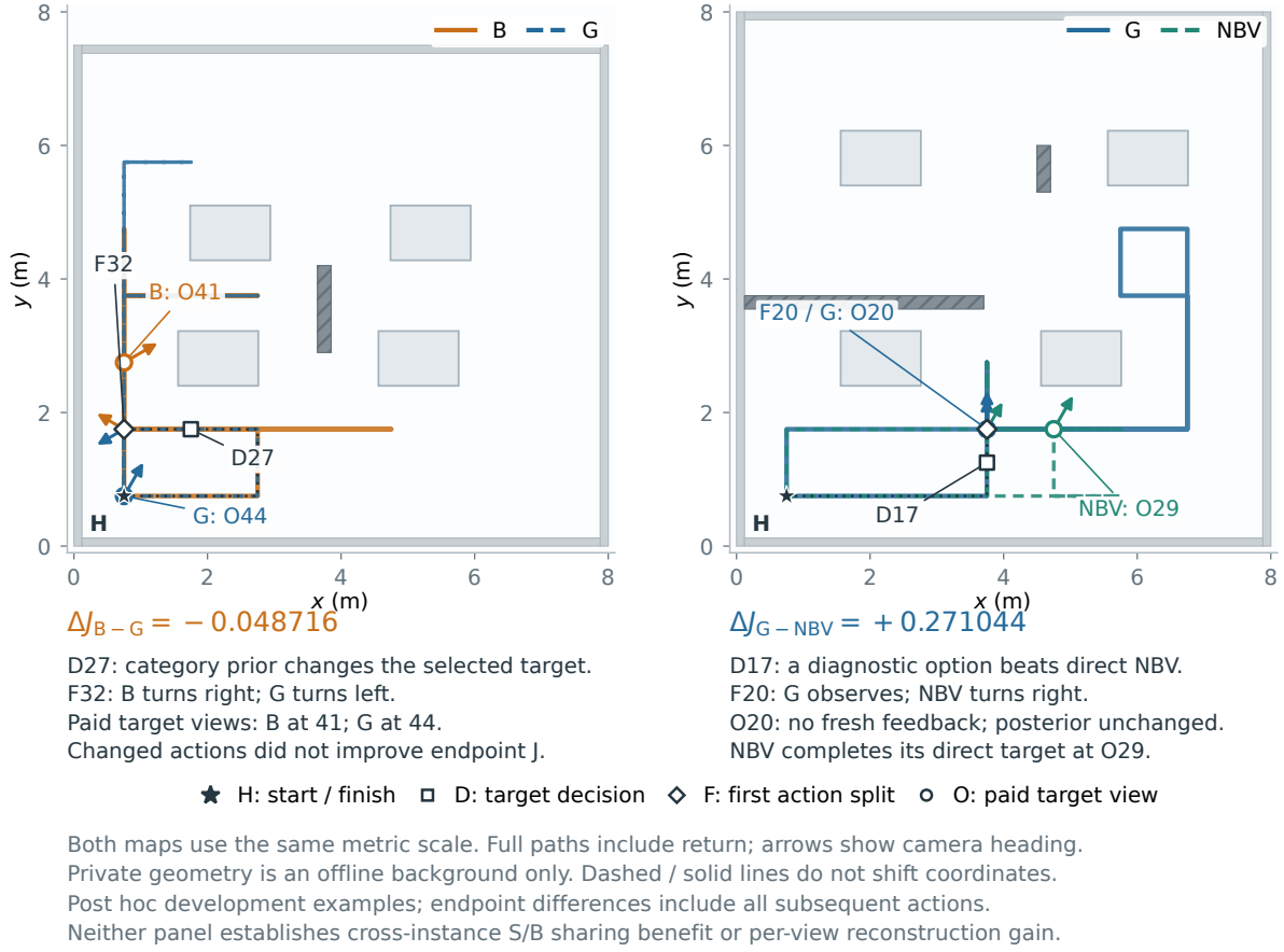
Figure 8 Two post hoc development mechanisms at a common metric scale, including complete returns. AISLE B/G select different targets at step 27 and first execute different actions at 32; J(B) - J(G) = -0.048716 . CELL G/NBV select different options at 17 and diverge at 20; J(G) - J(NBV) = +0.271044 , without fresh feedback at G's diagnostic completion. D/F/O/H mark decision, first action divergence, observation completion, and home. Geometry is offline context. Later routes also differ, so endpoint contrasts are not isolated first-view effects.
