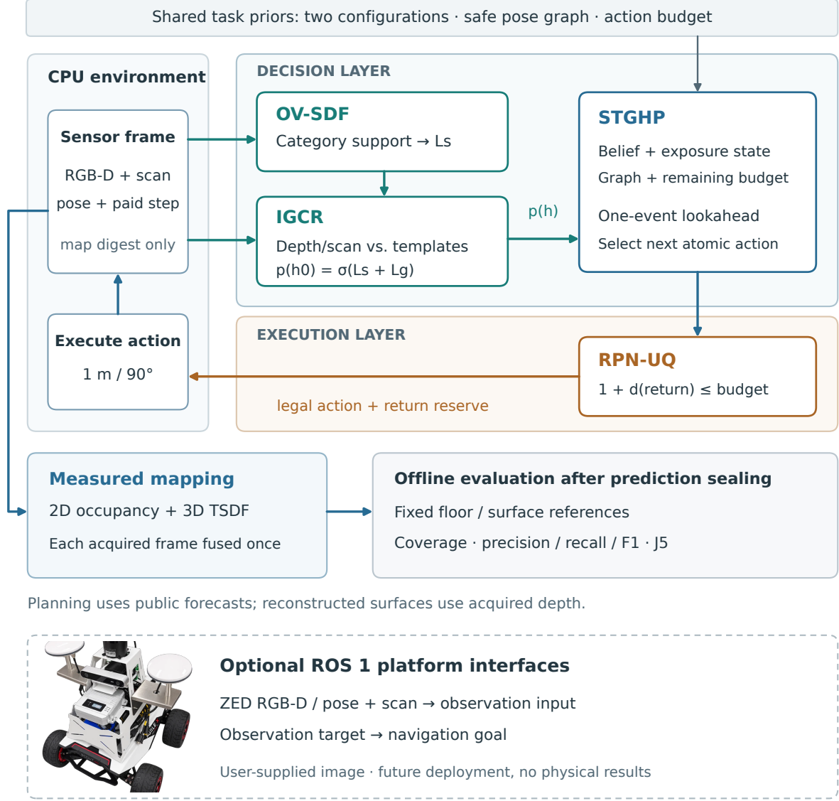
Figure 2 Platform interfaces, the local binary implementation of the four-module CPU loop, and separate mapping and evaluation. OV-SDF and IGCR jointly update configuration belief; STGHP selects the next atomic action for RPN-UQ to check before execution and new observation. Public templates support belief and planning, while TSDF fuses measured depth and ground truth enters only evaluation of sealed outputs. The unchanged user-supplied robot image illustrates prospective ROS 1 interfaces, while the vector diagram describes the executed CPU loop. All performance results use simulation.
