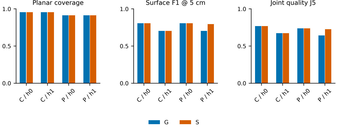
Figure 22 Coverage, surface F1 at 5 cm and joint quality for all four paired conditions. C/P denote column/partition; paired coverage remains equal. The three ties and one positive condition are retained on common 0–1 axes, without treating methods or configurations as independent layout replicates.
