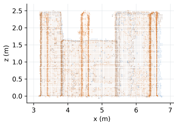
Slot 0 / A side (complex) XZ elevation
