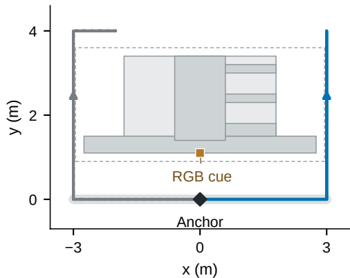
(a) Saved scene and executed paths
