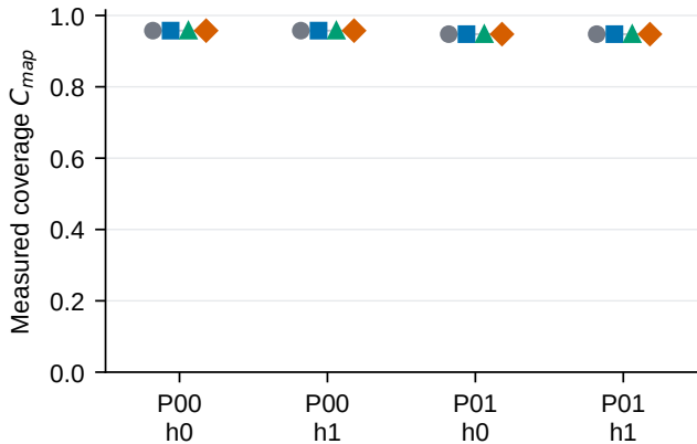
a Coverage
