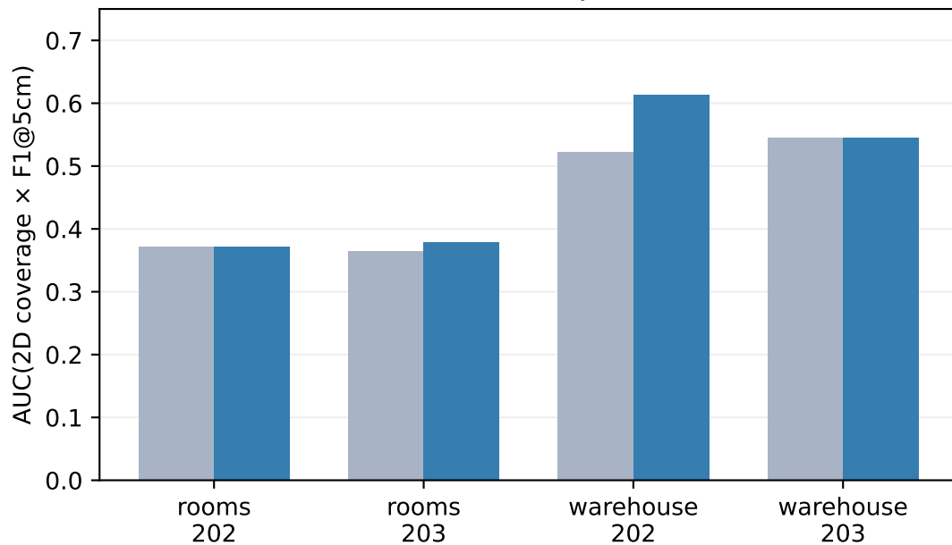
occluded objects
