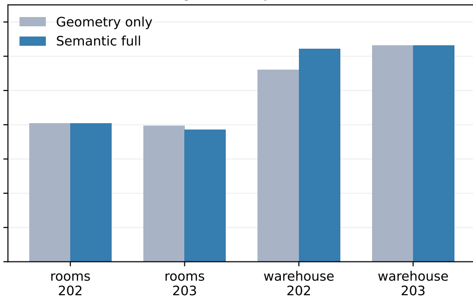
generic objects
