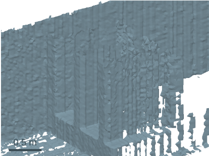
P00 / h1 S ribbed-side detail
