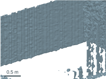
P00 / h1 G ribbed-side detail
