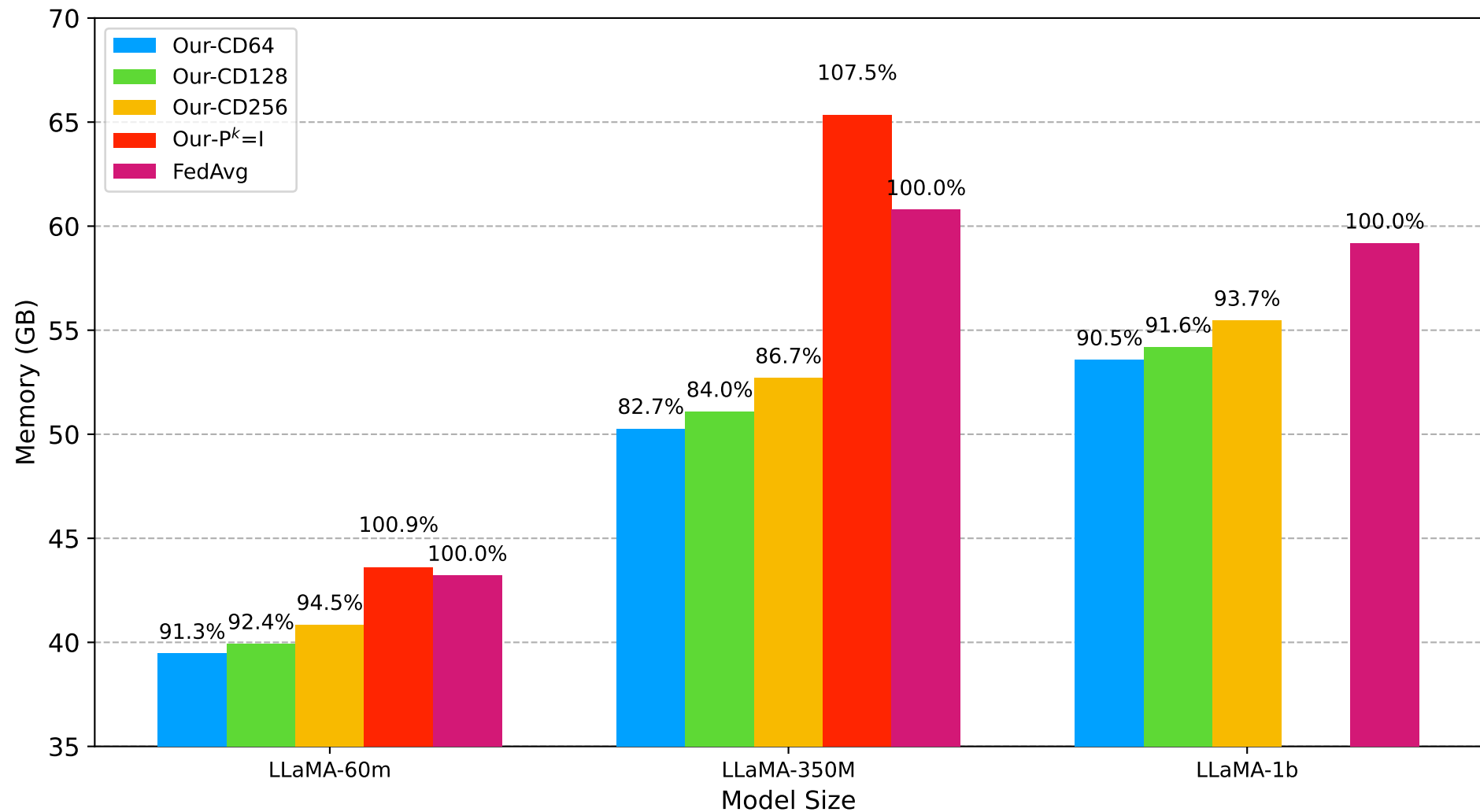
Memory Usage Comparison of Different Models and Methods
