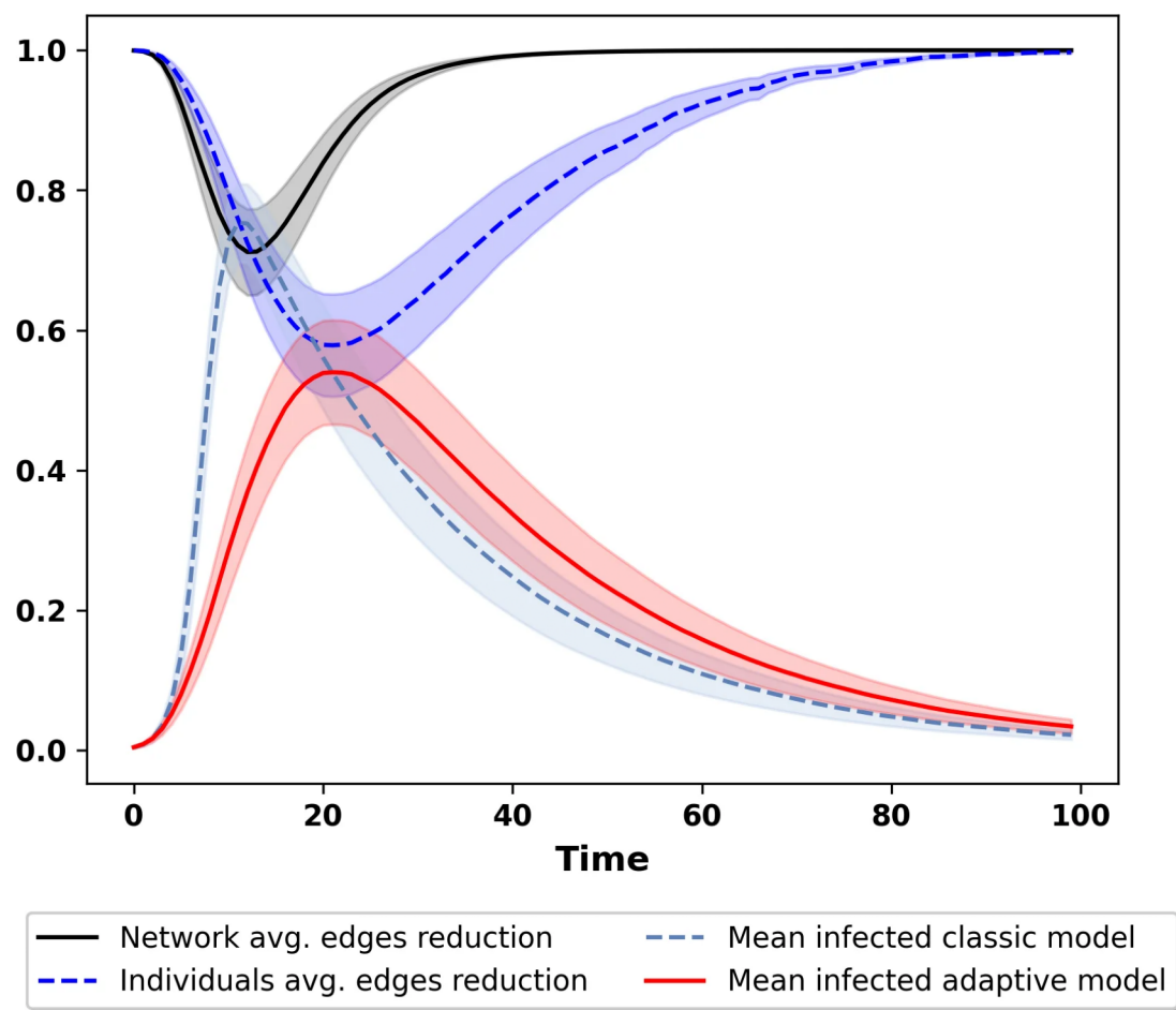
A) Global and local behavioral responses/Disease Prevalence
