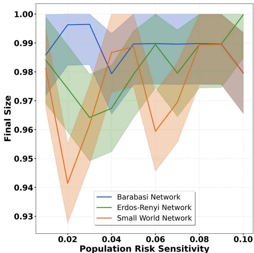
C) Final size vs sensitivity parameter for each network topology
