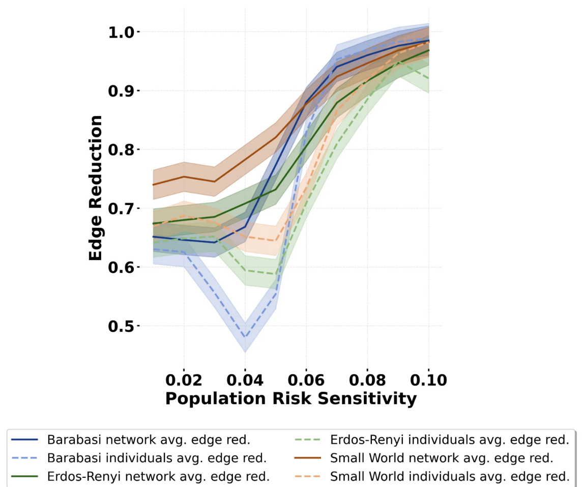
D) Avg min network and individual edge reduction vs sensitivity parameter for each network topology
