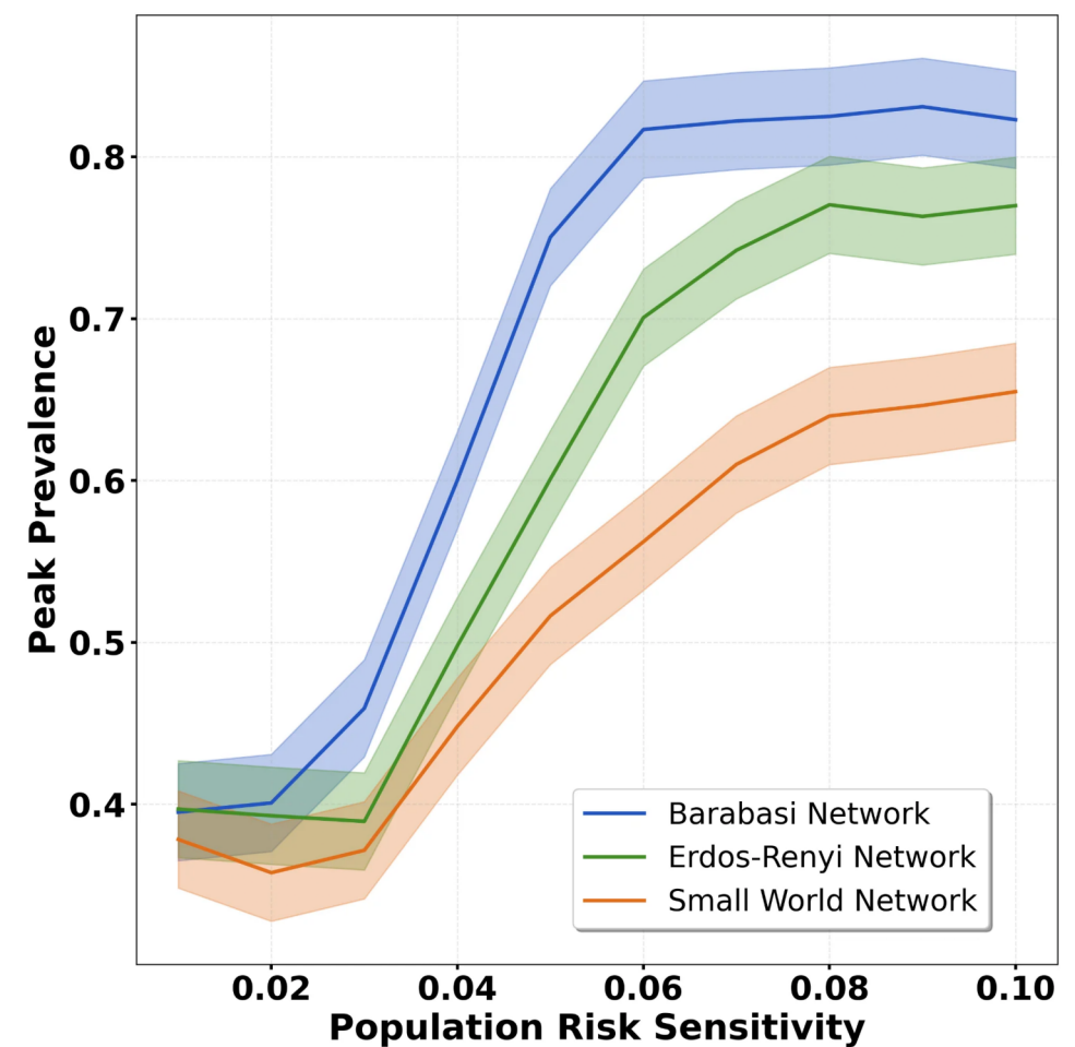
B) Prevalence peak size vs sensitivity parameter for each network topology
