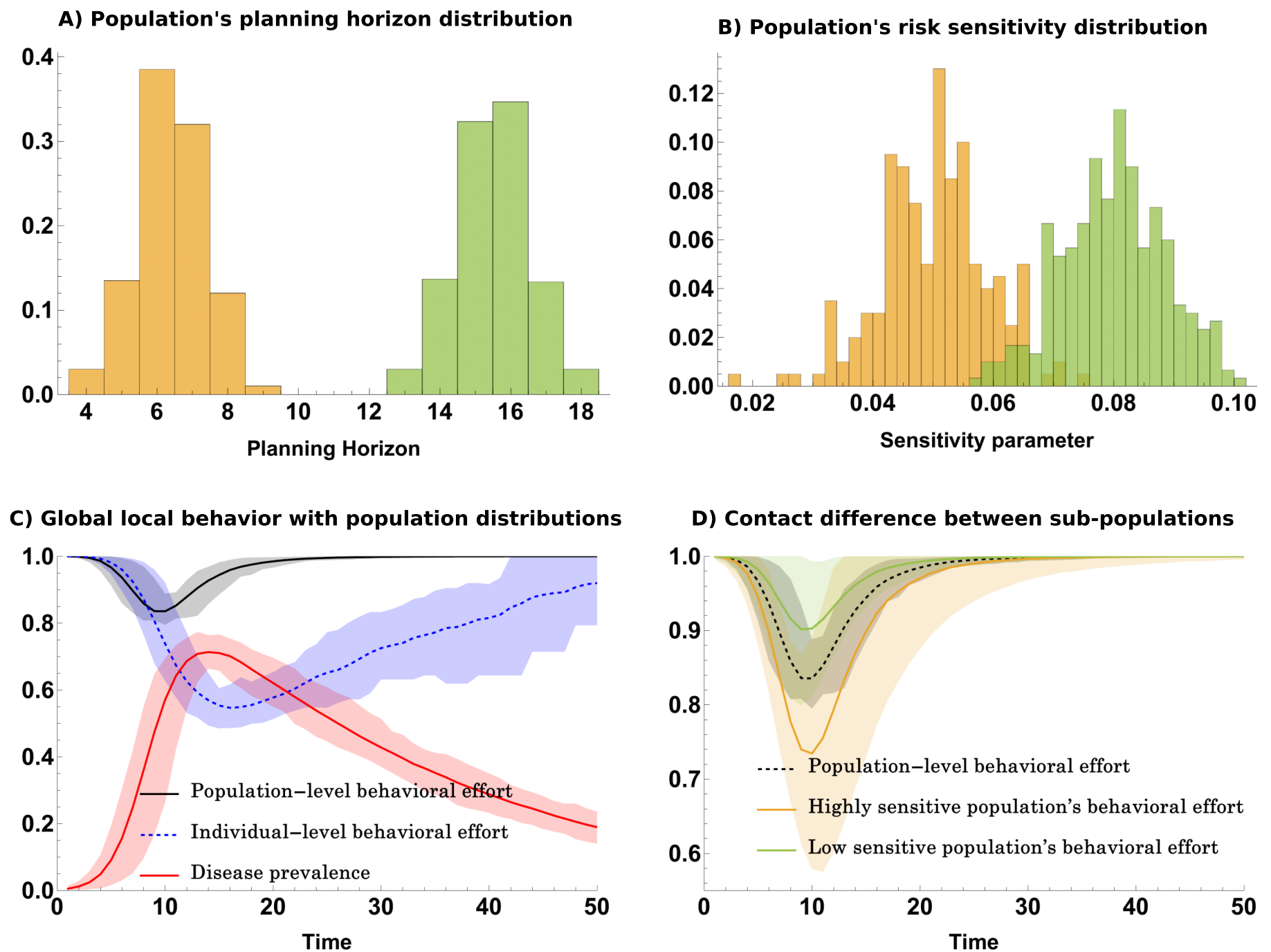
Fig. 4. (Panels A-B) Distributions of behavioral parameters for two sub-populations. In yellow, a sub-population with lower planning horizon and utility curvature parameter, representing individuals with higher sensitivity to disease progress. In green, a sub-population with higher parameter values, resulting in lower sensitivity. (Panel C) The global/local behavior effort lag persist even when heterogeneity in adaptive behavior parameters is introduced. (Panel D) Contact dynamics over the epidemic period for the high- and low-sensitivity populations, as well as the total population.
