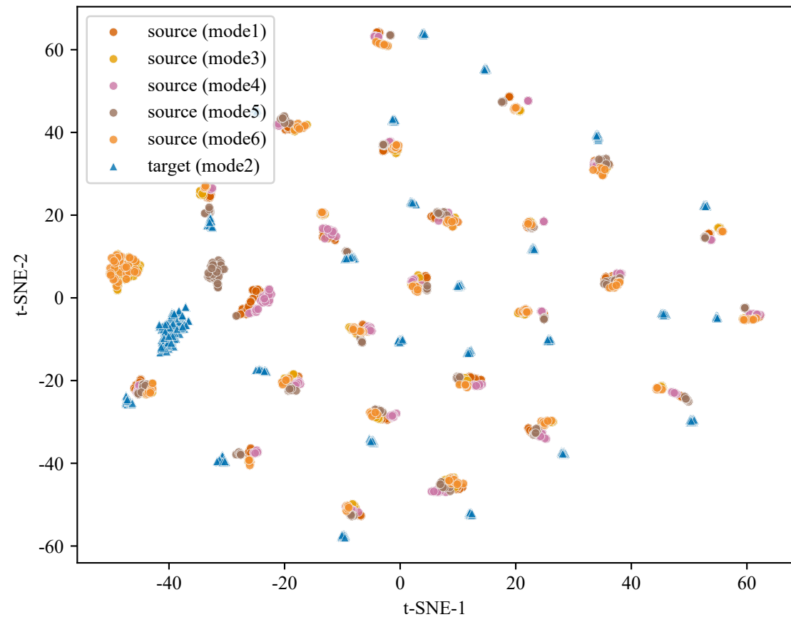
Domain Fusion t-SNE
