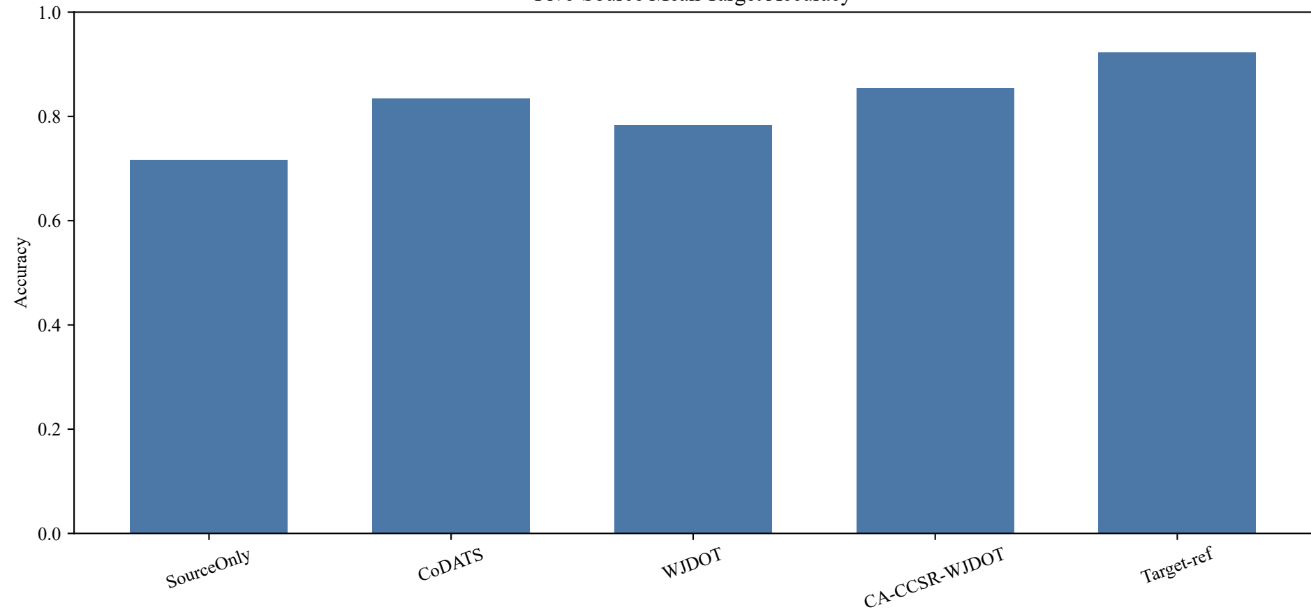
Five-Source Mean Target Accuracy
