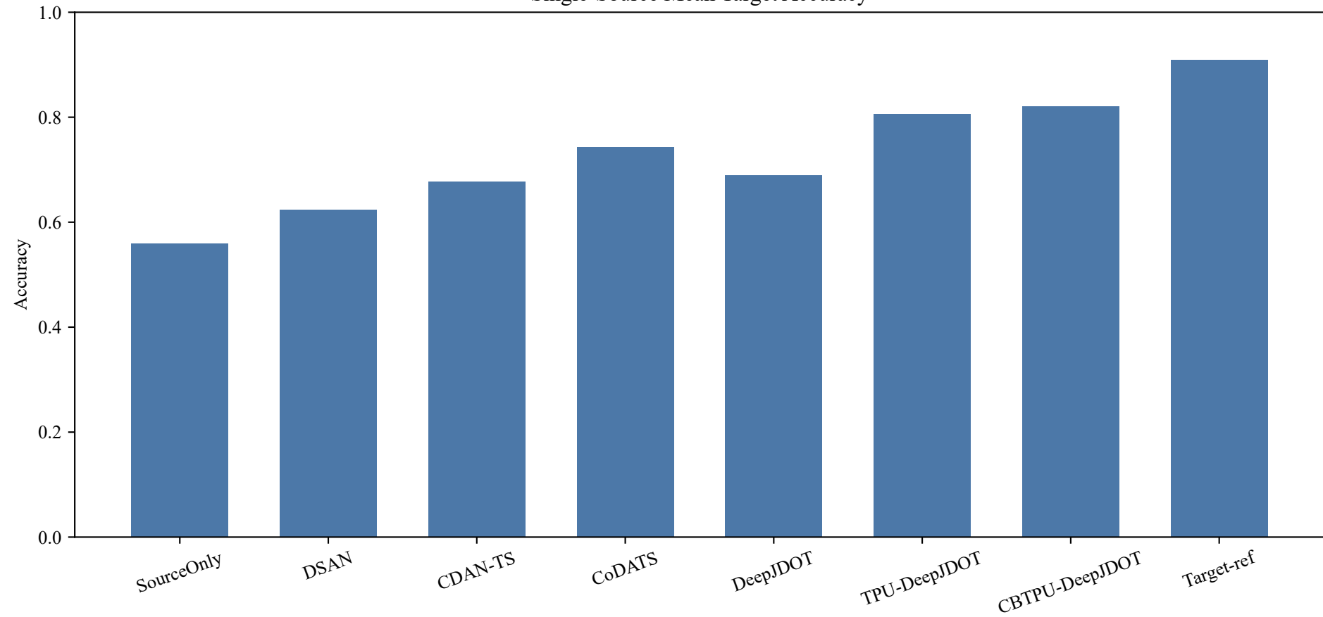
Single-Source Mean Target Accuracy
