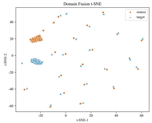
(b) DeepJDOT
