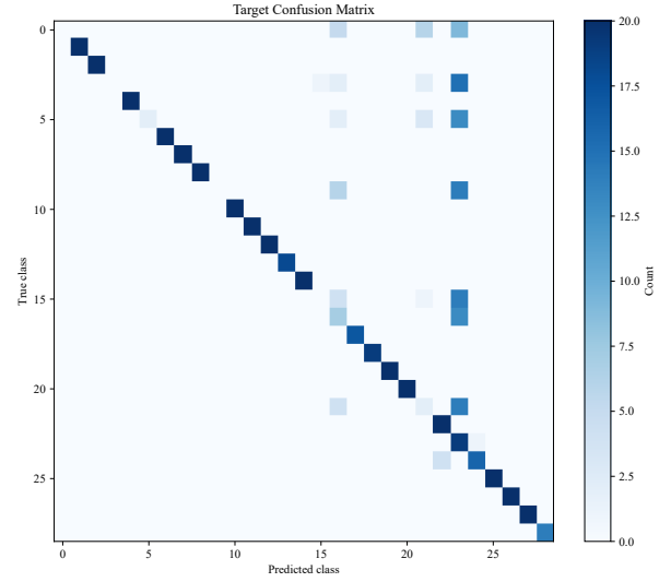
(b) DeepJDOT
