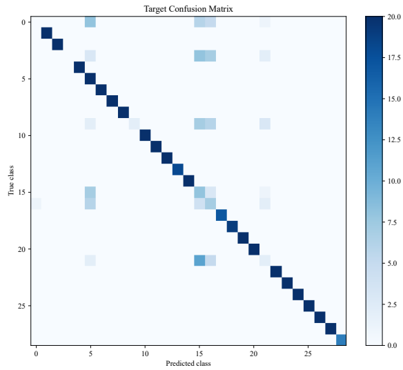
(c) TPU-DJDOT
