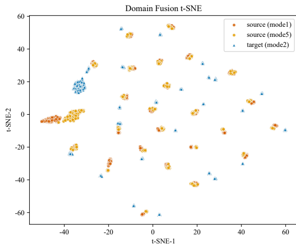
(c) WJDOT
