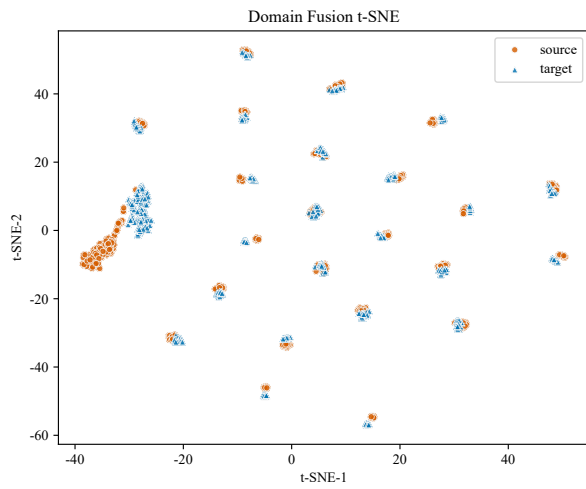
(c) TPU-DJDOT
