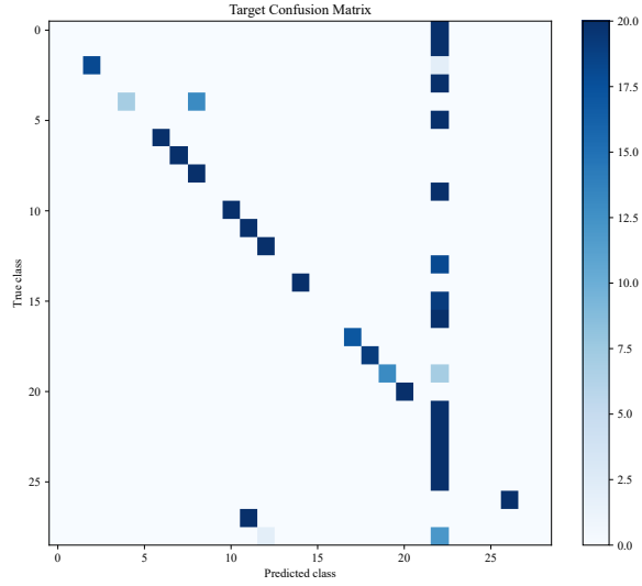
(a) SourceOnly
