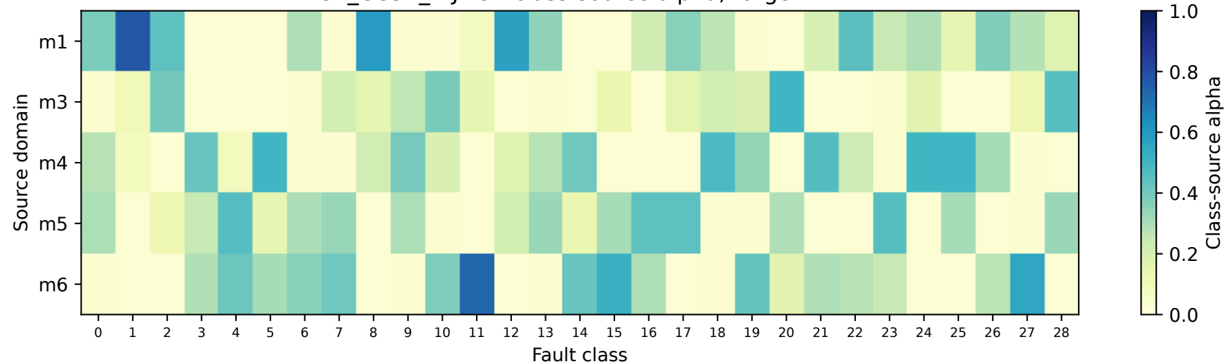
CA_CCSR_WJDOT class-source alpha, target m2
