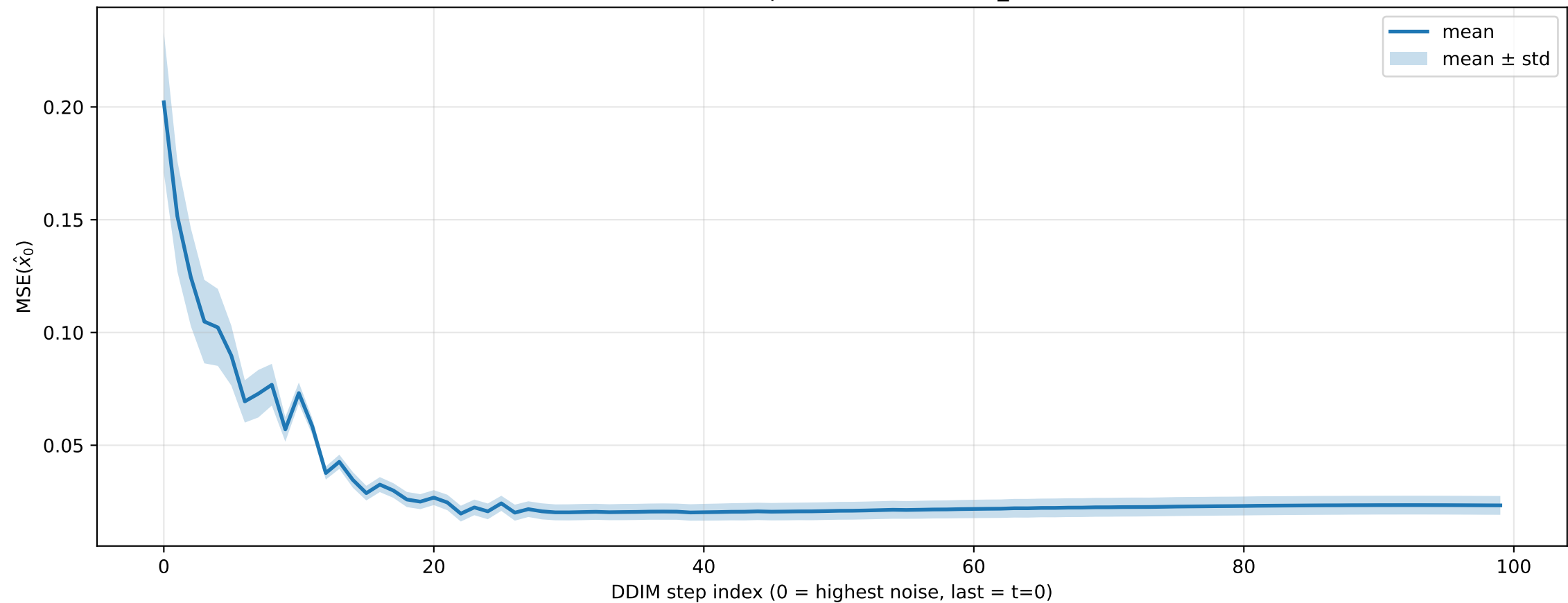
Per-Timestep MSE of Predicted x_0
