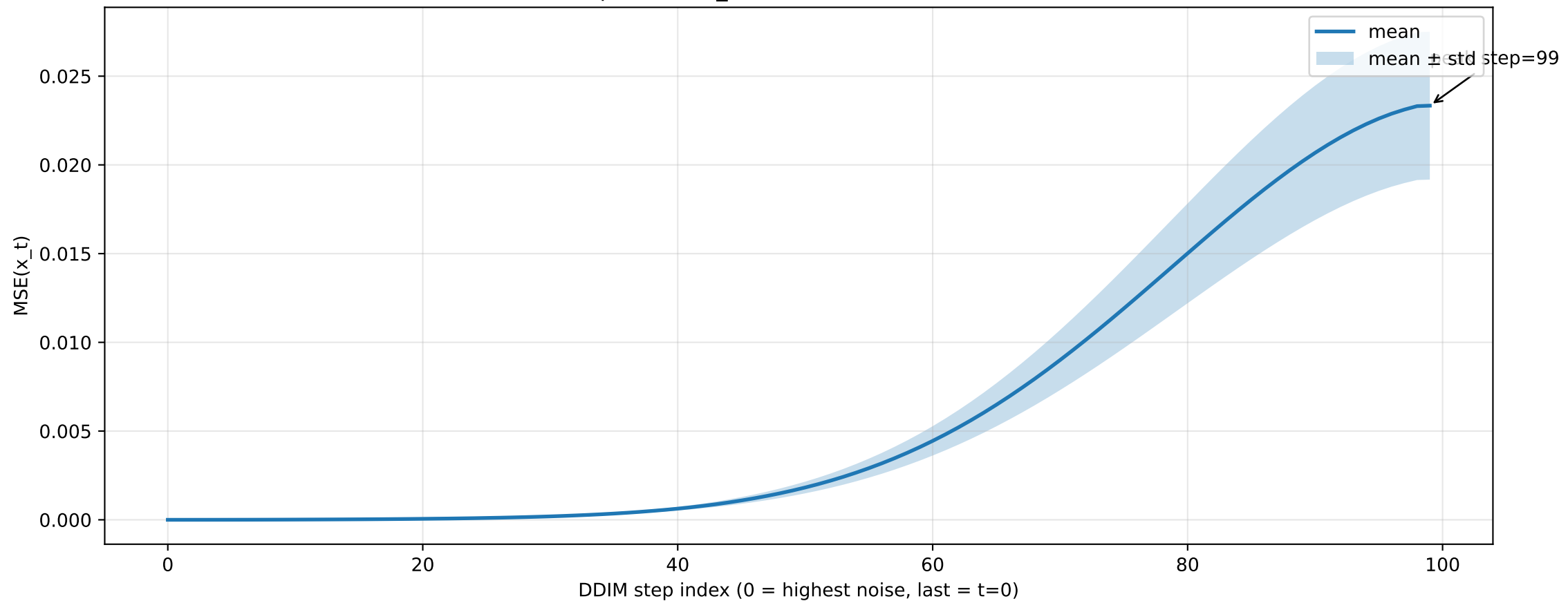
Per-Timestep MSE of x_t : Diff-AE (FP32) vs Q-DiffAE (W8A8)
