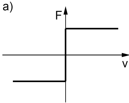
Figure 1: The change of friction with respect to velocity
