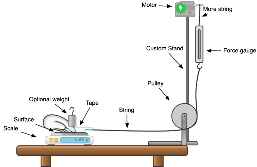
Figure 5: The experimental setup for measuring Coulomb and static friction
