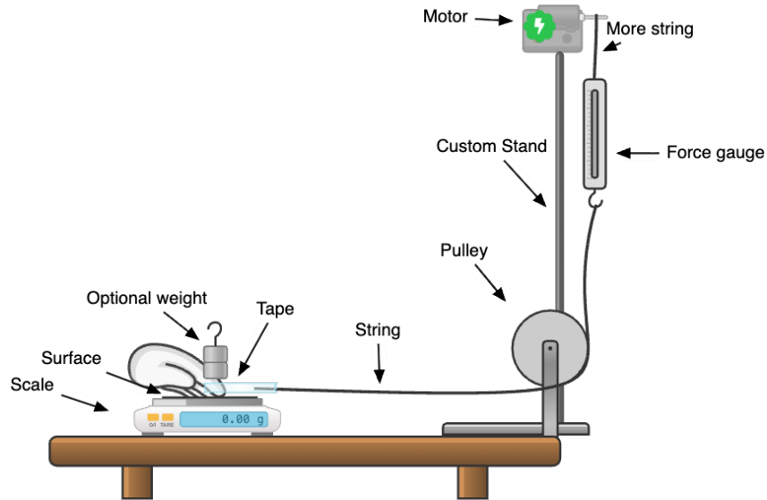
Figure 8: The experimental setup for measuring Coulomb and static friction
