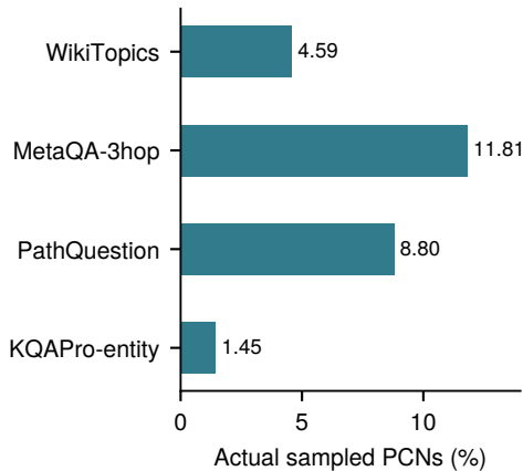
a Training conflict prevalence
