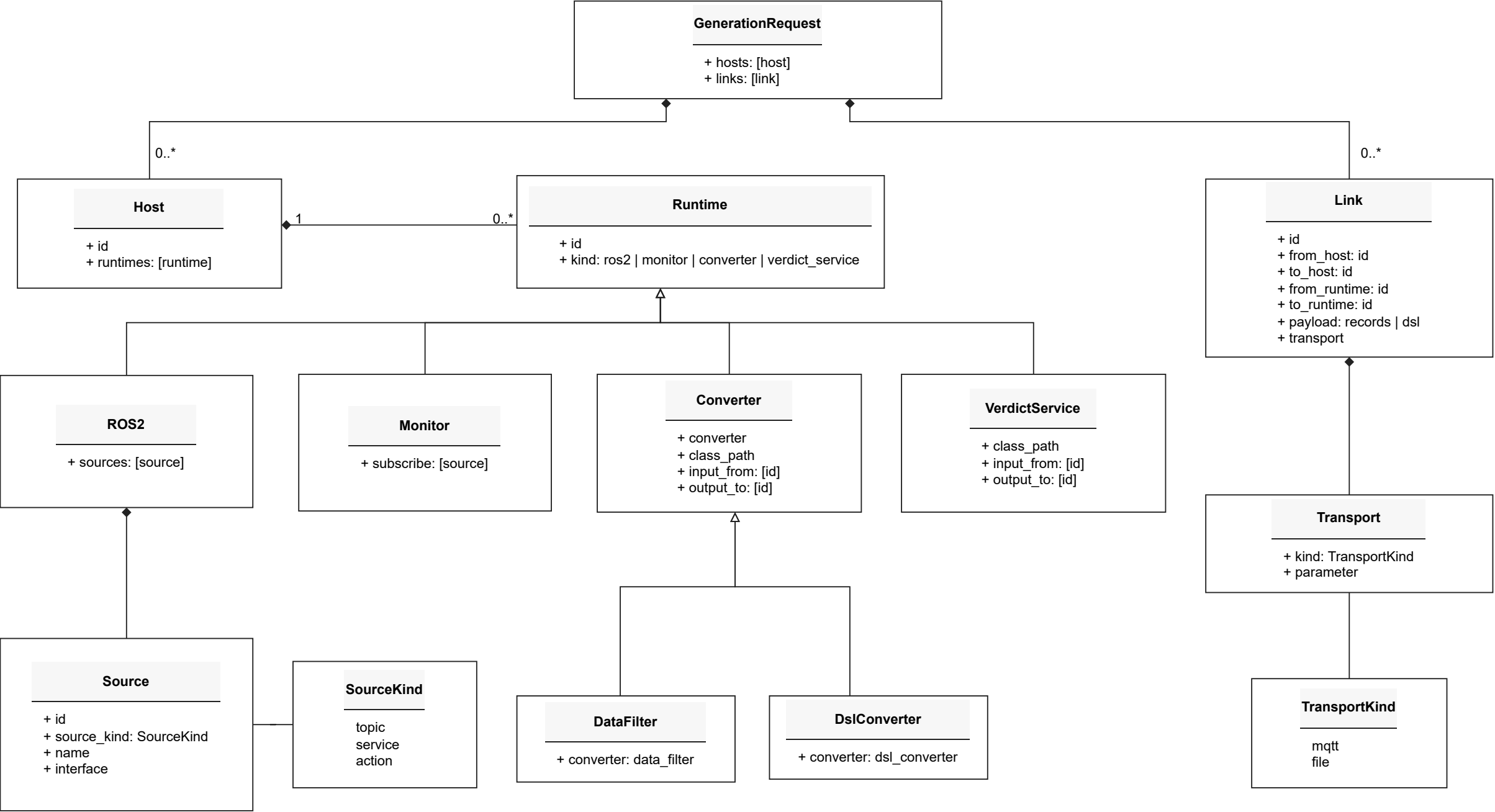
UML Class Diagram for Host Runtime Link JSON
