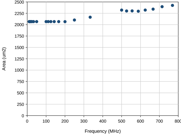
Figure 1: Area, frequency for unpipelined mac (MET).
