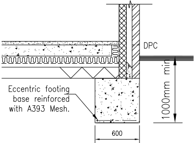
BOUNDARY SECTION Scale 1:50
