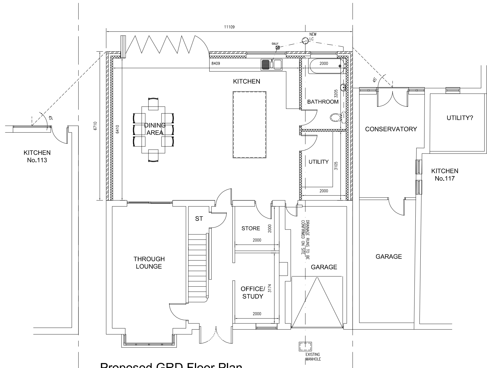
Proposed GRD Floor Plan
