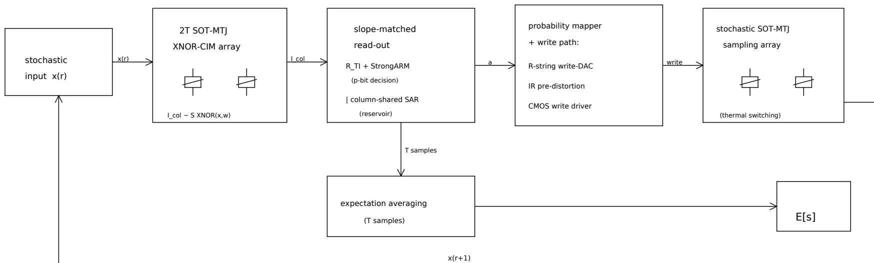
sMTJ-PBNN closed-loop forward (circuit-accurate architecture)
