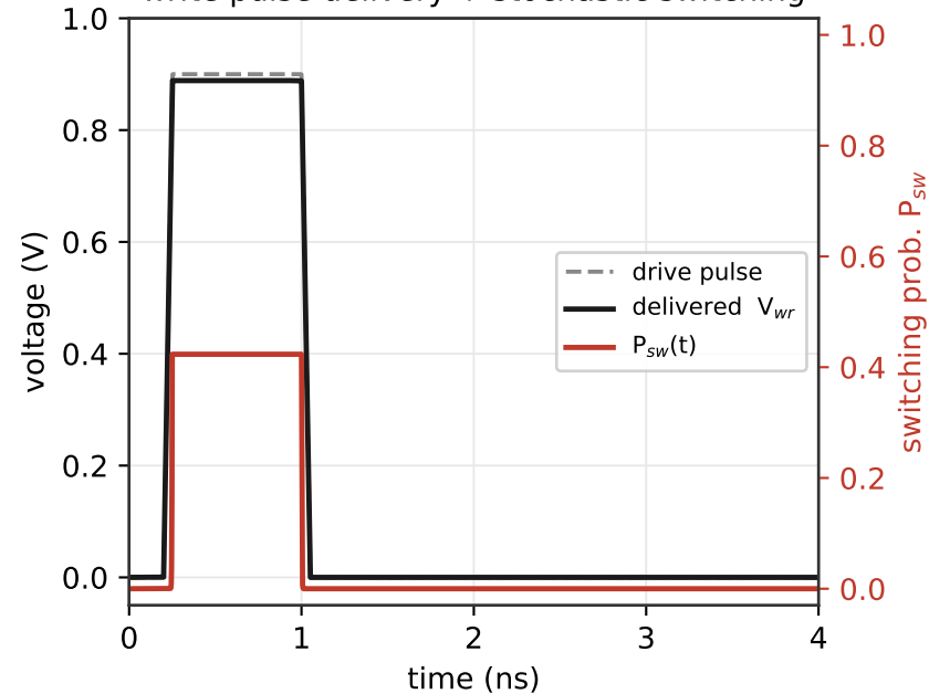
write pulse delivery + stochastic switching
