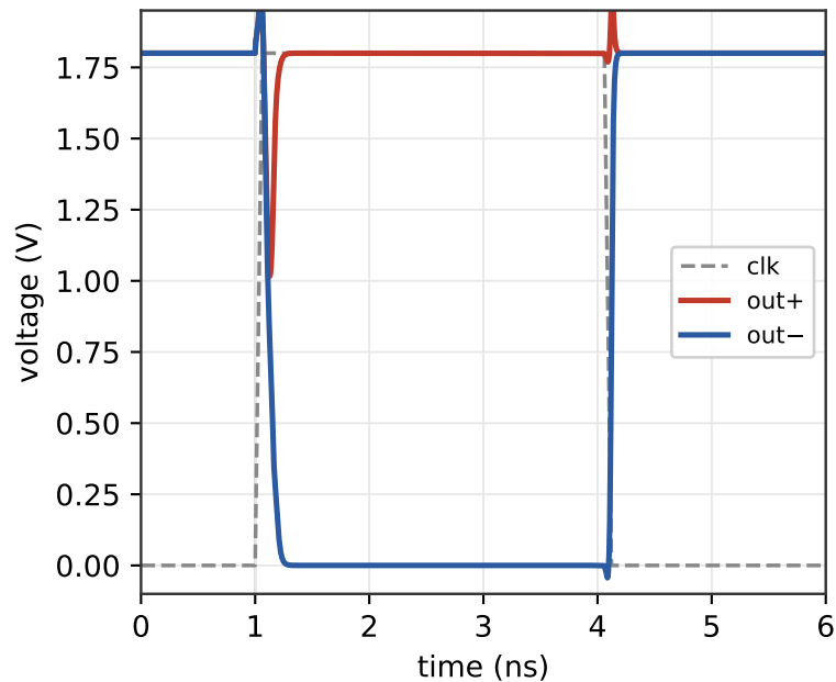
StrongARM regeneration (10 mV input)
