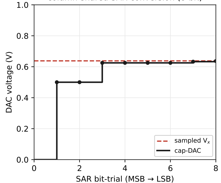
column-shared SAR conversion (8-bit)
