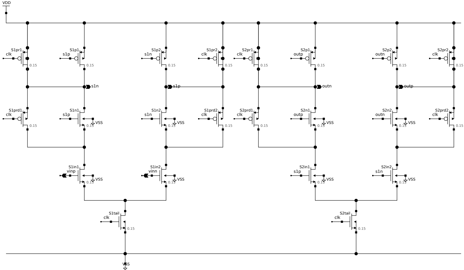
offset Vo1-4 injected on stage-1 input/latch gates (testbench)
