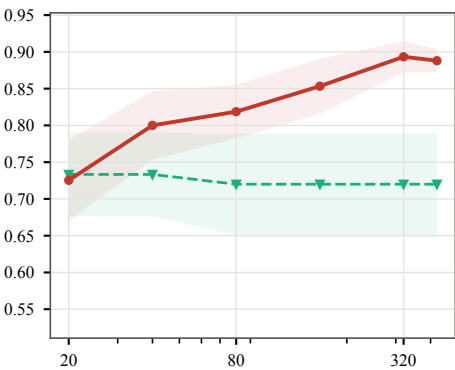
MT-Bench, n_L = 160 Kendall's \tau , held-out ranking
