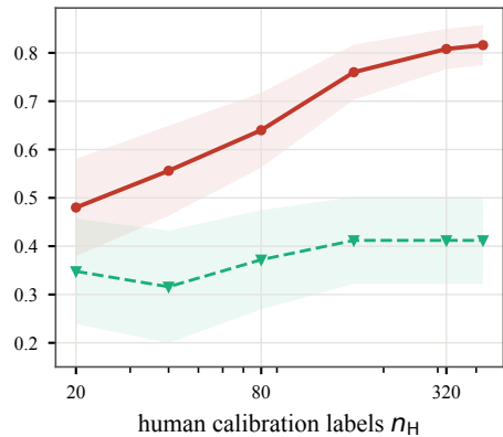
PandaLM, n_L = 100 Kendall's \tau , held-out ranking
