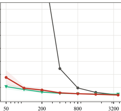
large6 (203B)
