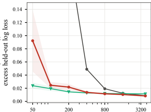
small6 (36.5B)
