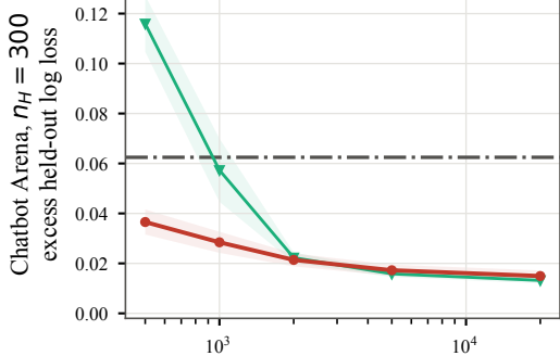
small6 (36.5B)
