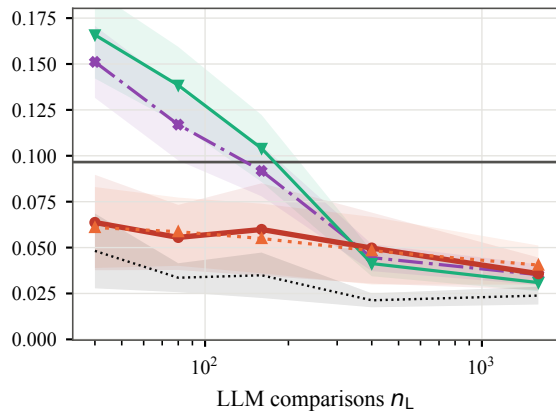
MT-Bench, 5 biased judges, n_H=80
