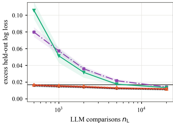
Chatbot Arena, 5 biased judges, n_H=1000
