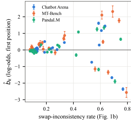
(c) judge-level position effects
