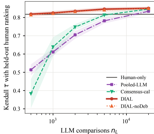
(a) Arena, 5 biased judges, n_0 = 1000
