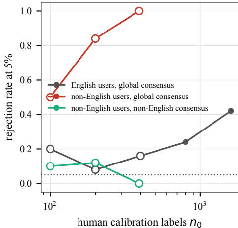
(b) test of S_0 = \alpha\mu
