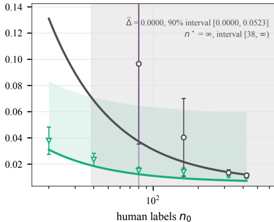
MT-Bench (pilot n_0 = 80 )
