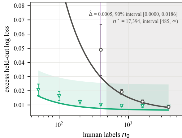
Chatbot Arena (pilot n_0 = 400 )
