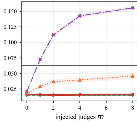
(b) position-only, log loss
