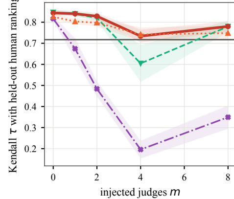
(c) anti-consensus, Kendall \tau
