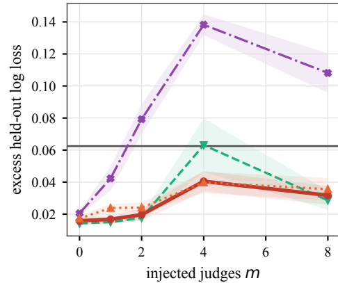
(a) anti-consensus, log loss
