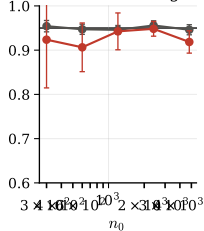
95% CI coverage
